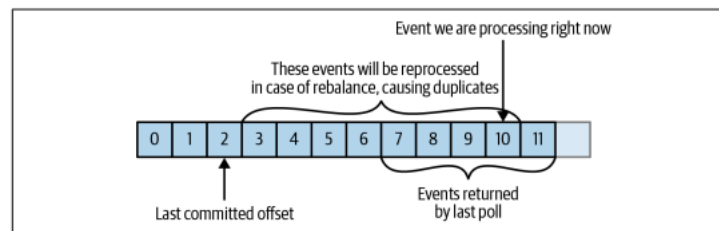
Figure 4-8. Reprocessed messages
