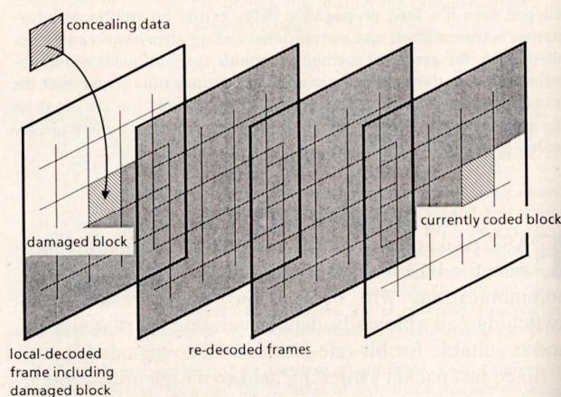
Fig. 2. Illustration of Method B.
