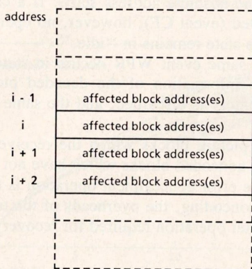
Fig. 5. Structure of block relation table.
