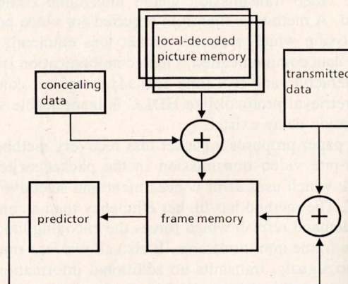
Fig. 3. Redecoding algorithm of Method B.
