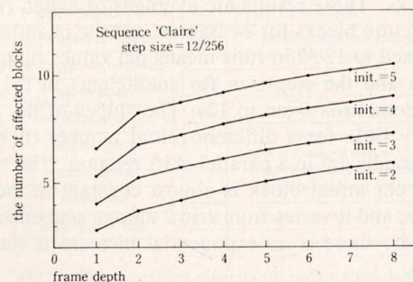
Fig. 9. The number of affected blocks after loss of consecutive picture blocks.
