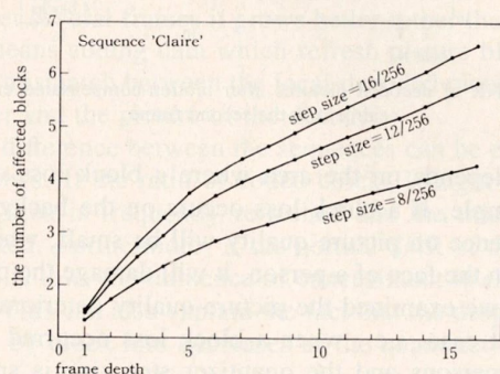
Fig. 8. The number of affected blocks after loss of one picture block.
