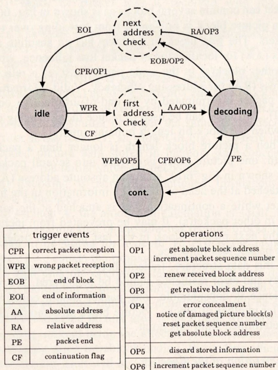
Fig. 7. State transition diagram for packet receiving.
