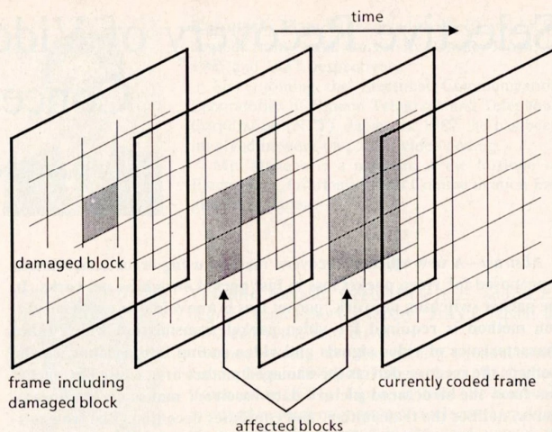
Fig. 1. Illustration of Method A.
