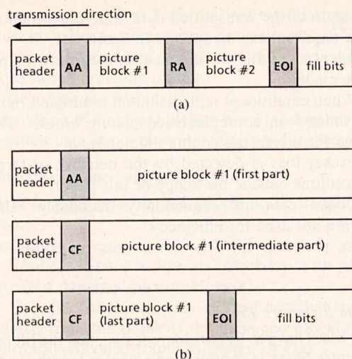
Fig. 6. Structure of data packing. (a) Picture block length < packet length. (b) Picture block length > packet length.
