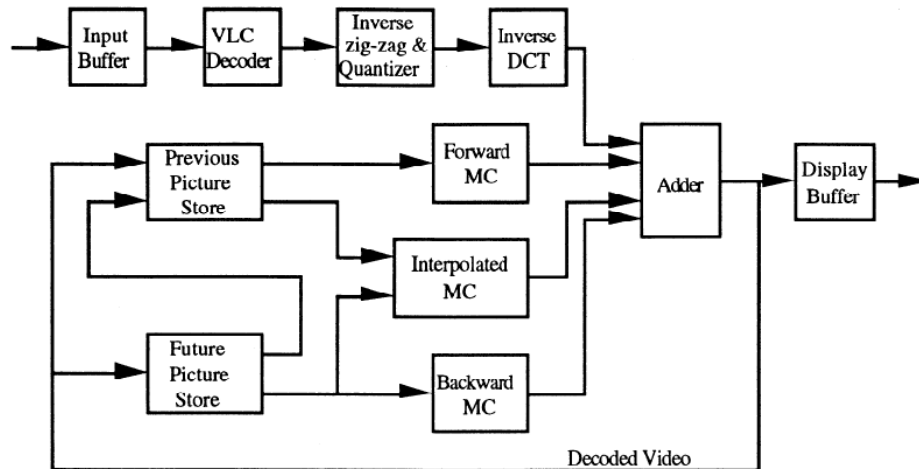
Figure D.7 -- Simplified decoder block diagram
