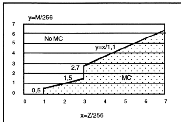
Figure D.33 -- Characteristic MC/No MC
