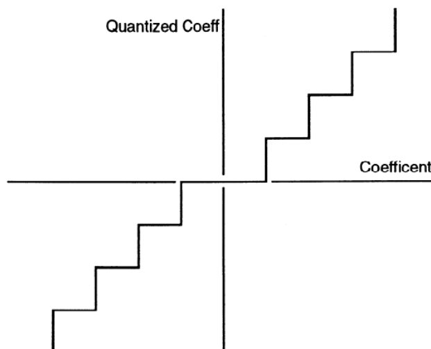
Figure D.35 -- Dead zone quantizer characteristic
