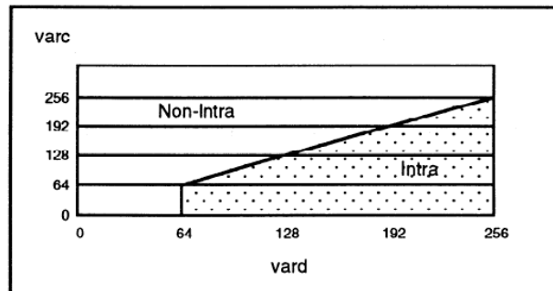
Figure D.34 -- Characteristic intra/non-intra
