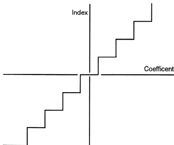
Figure D.29. -- Uniform quantizer characteristics
