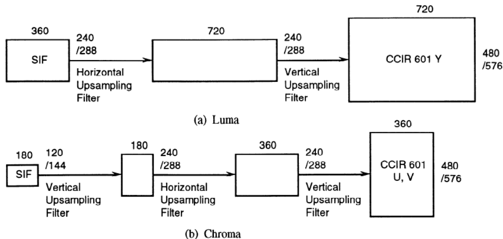
Figure D.41 -- Simplified decoder block diagram
