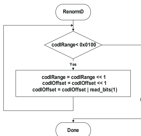
Figure 9-4 – Flowchart of renormalization
