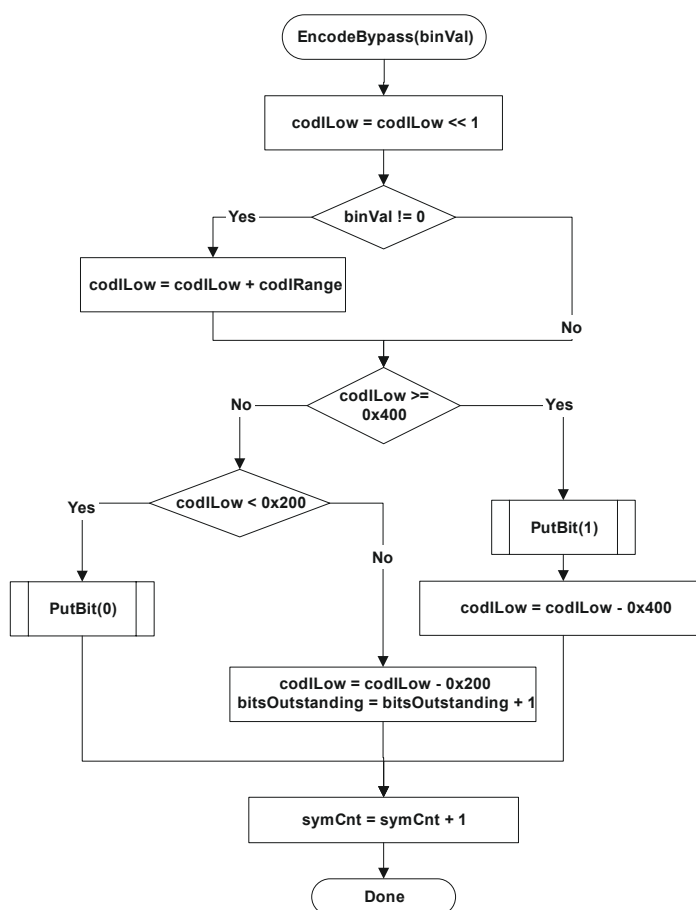
Figure 9-10 – Flowchart of encoding bypass
