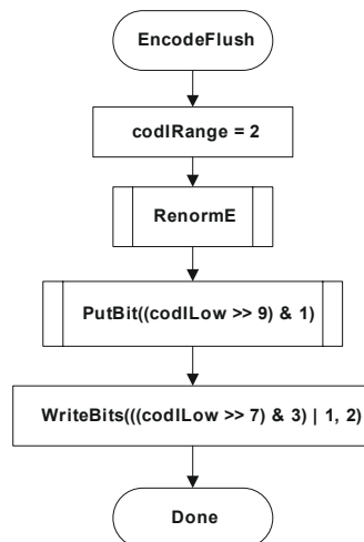
Figure 9-12 – Flowchart of flushing at termination
