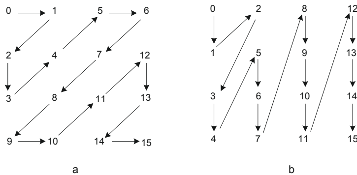
Figure 8-8 – a) Zig-zag scan. b) Field scan
