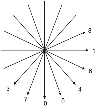
Figure 8-1 – Intra_4x4 prediction mode directions (informative)
