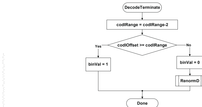
Figure 9-6 – Flowchart of decoding a decision before termination
