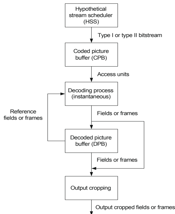
Figure C-2 – HRD buffer model
