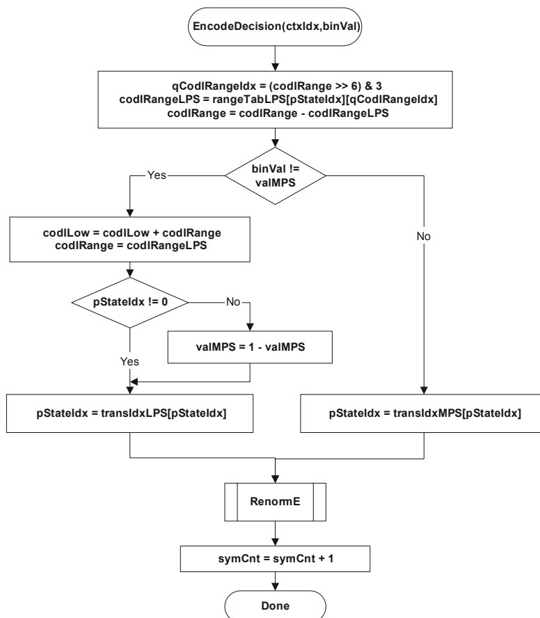
Figure 9-7 – Flowchart for encoding a decision
