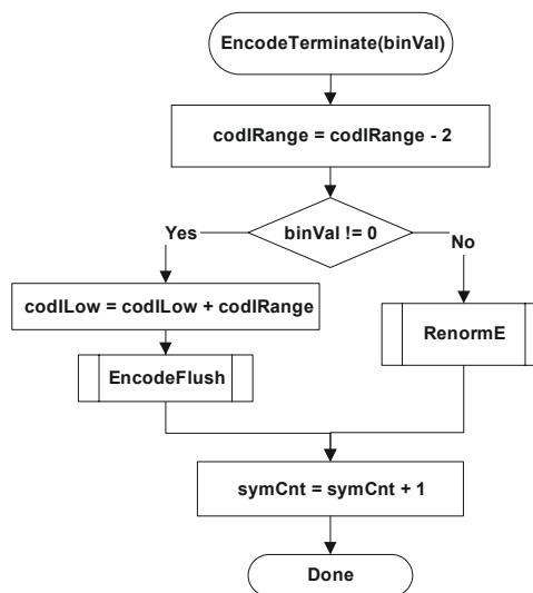
Figure 9-11 – Flowchart of encoding a decision before termination
