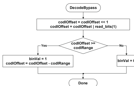
Figure 9-5 – Flowchart of bypass decoding process
