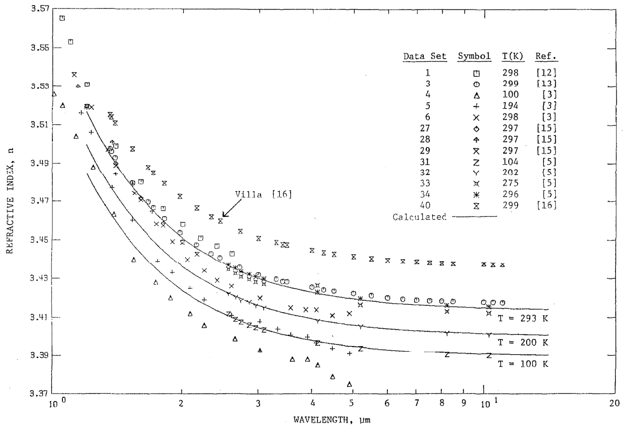
FIGURE 3. SELECTED EXPERIMENTAL REFRACTIVE INDEX OF SILICON (Wavelength Dependence)
