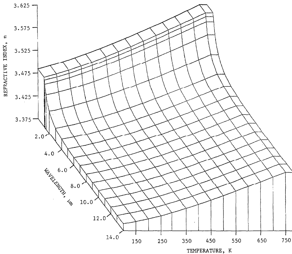
FIGURE 8. RECOMMENDED n - \lambda - T DIAGRAM OF SILICON
