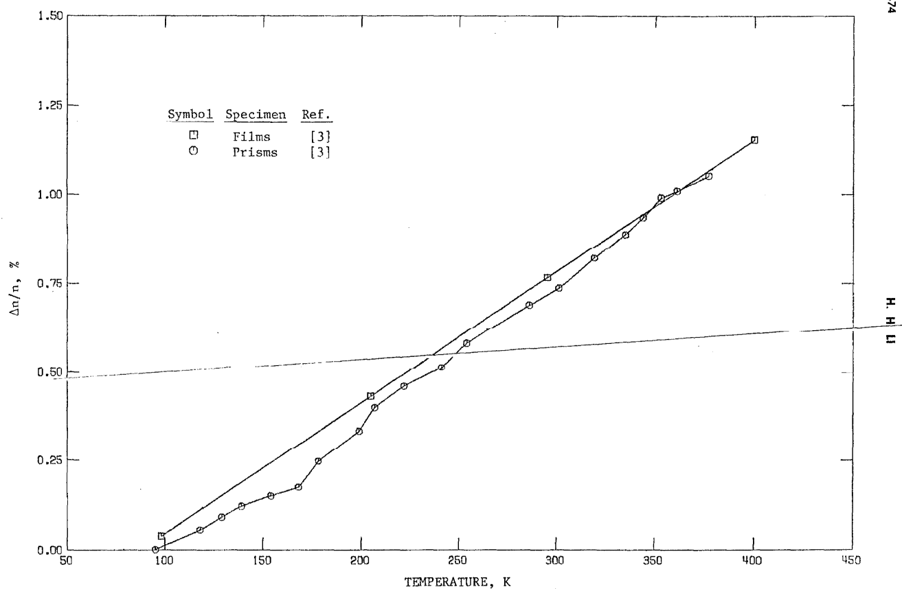
FIGURE 6. VARIATION OF REFRACTIVE INDEX OF SILICON WITH TEMPERATURE AT WAVELENGTH 3 \mu\text{m} [3]
