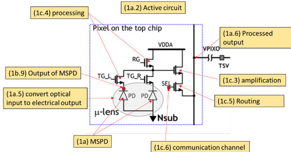
Ex. 14 (Samsung's 2PD Article) at Fig. 3 (annotated schematics of pixel circuit).
