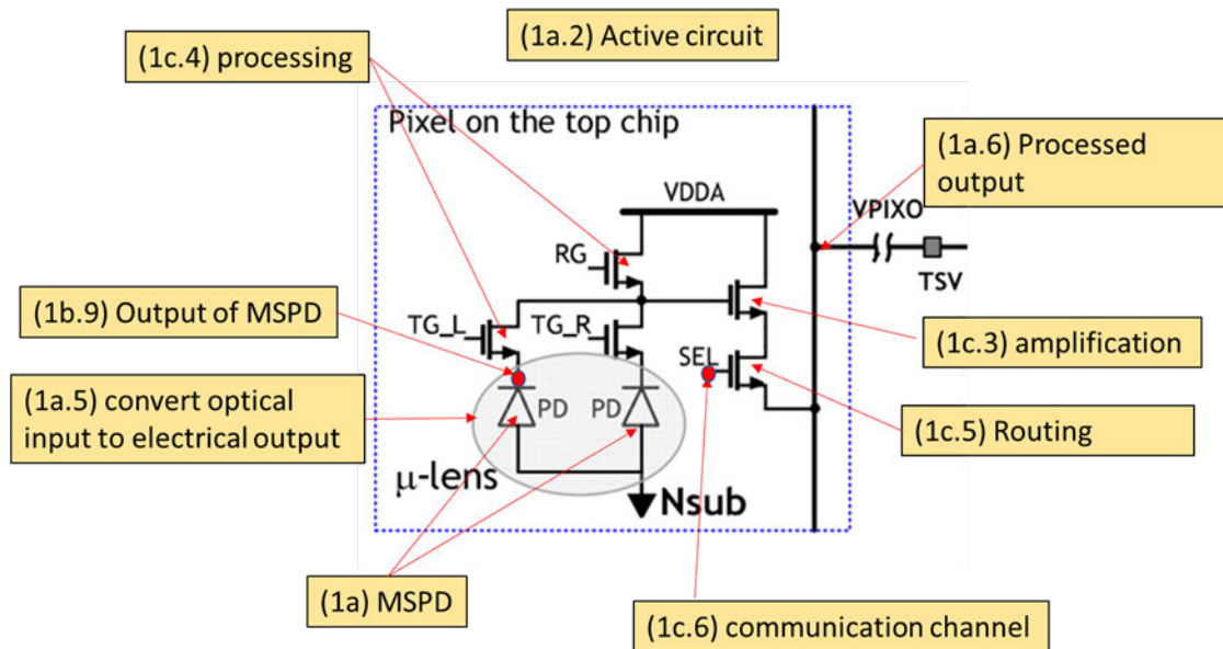
Ex. 14 (Samsung's 2020 2PD Article) at Fig. 3 (schematics of pixel circuit, annotated with claim elements of Claim 1 of the '700 Patent).
