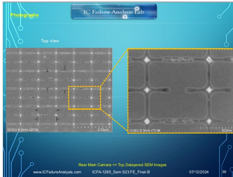
Ex. 25 (ICFA-1265) at Slide 30 (SEM images after the surface materials are mechanically polished away, revealing the top view of the semiconductor pixels).
