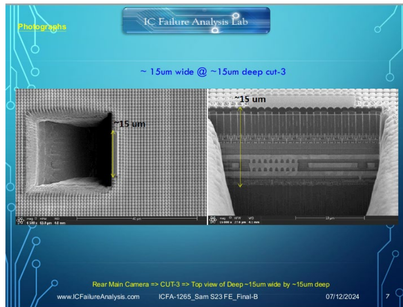
Ex. 25 (ICFA-1265) at Slide 7 (showing a portion of material removed by FIB to expose the cross-section of \sim 15\ \mu\text{m} wide and 15\ \mu\text{m} deep).
