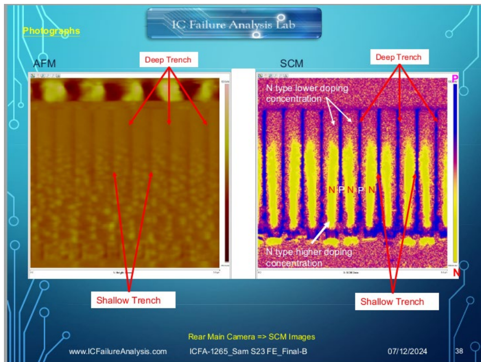
Ex. 25 (ICFA-1265) at Slide 38 (SCM images showing doping profile inside the pillars, where the yellow region is highly doped n-type, the blue region is highly doped p-type and the purple region is lightly doped n-type).
