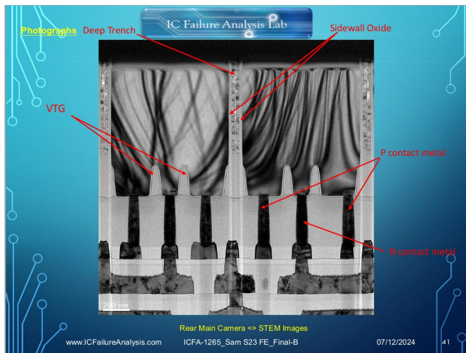
Ex. 25 (ICFA-1265) at Slide 41 (TEM showing VTG's (vertical transfer gates) are integrated into the photodetector; the P-contact and N contact facilitates reverse biasing of the photodetector).
