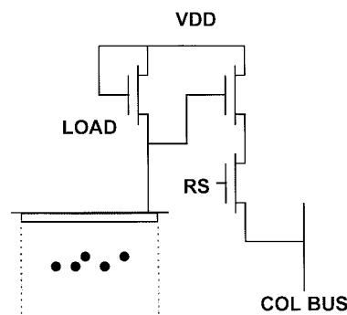
Fig. 9. Logarithmic pixel schematic circuit.
