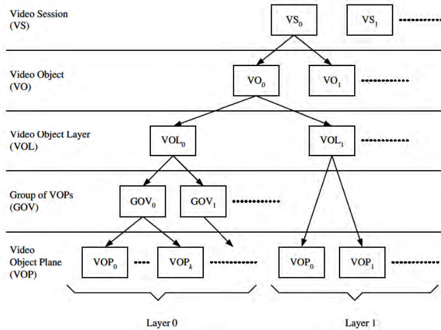
Figure 3.7: MPEG-4 video bitstream structure
