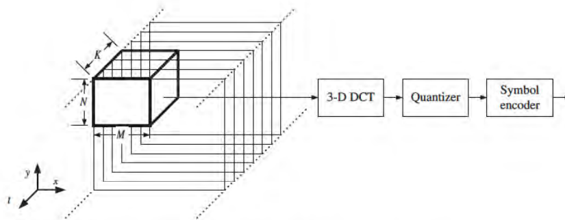
Figure 2.14: A 3-D transform coding system
