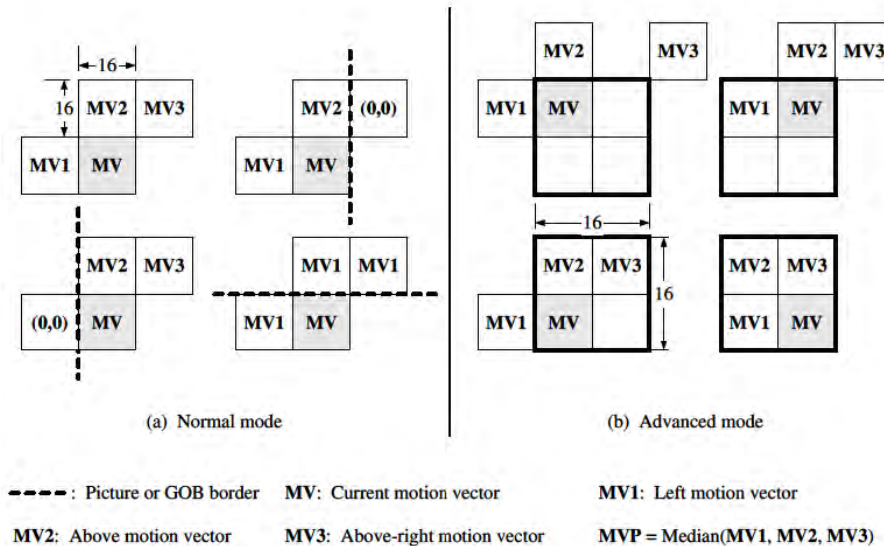
Figure 3.3: H.263 motion vector prediction
