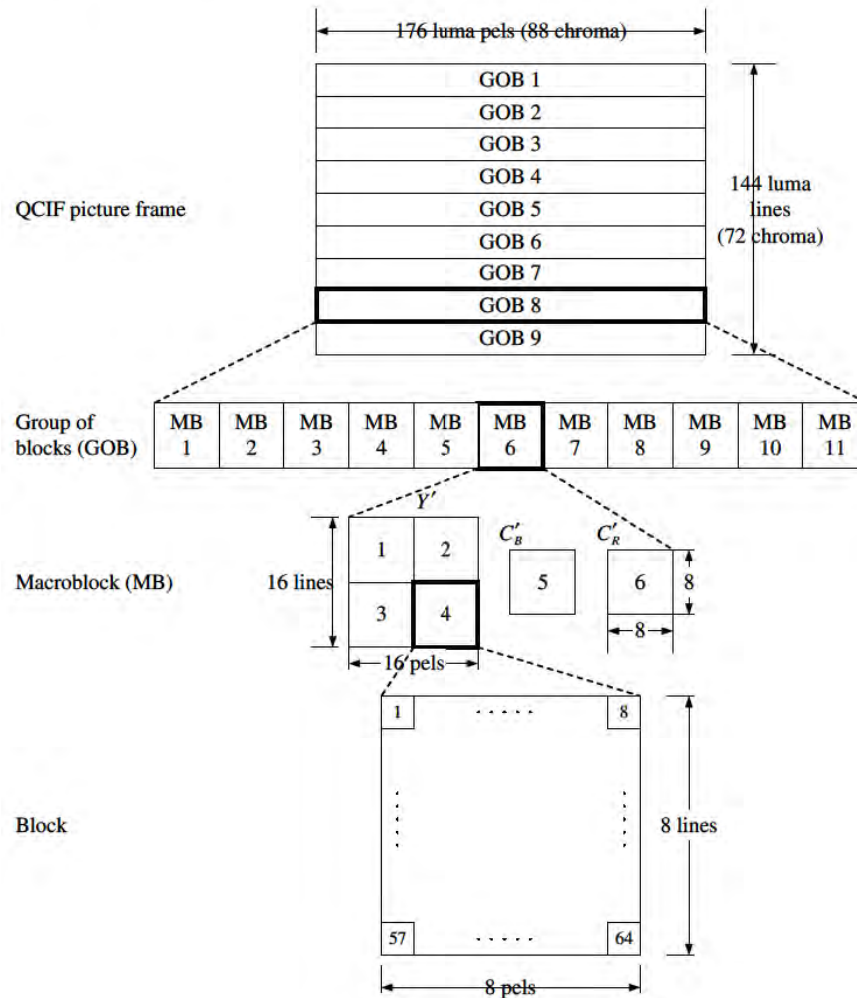
Figure 3.2: H.263 picture structure for a QCIF frame
