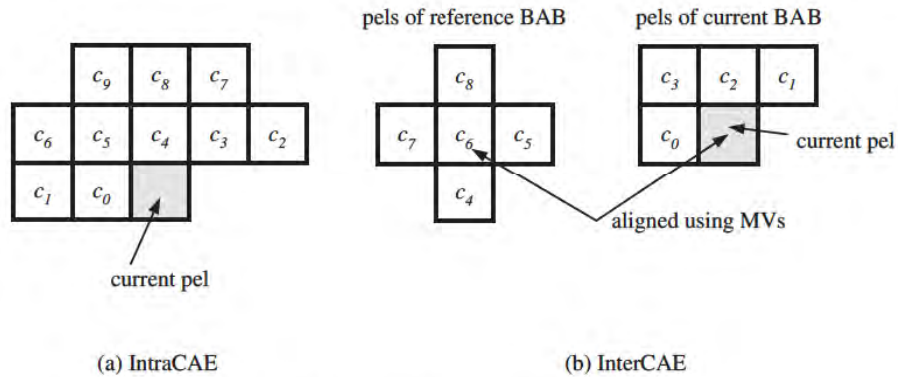
Figure 3.13: CAE templates in MPEG-4
