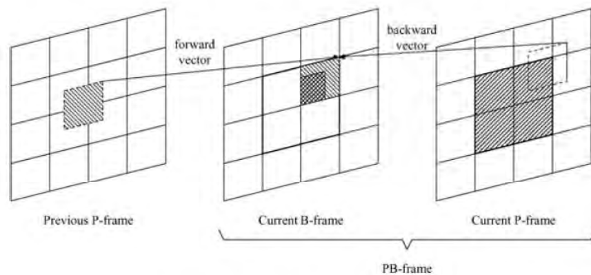
Figure 3.4: Prediction in PB-frames mode
