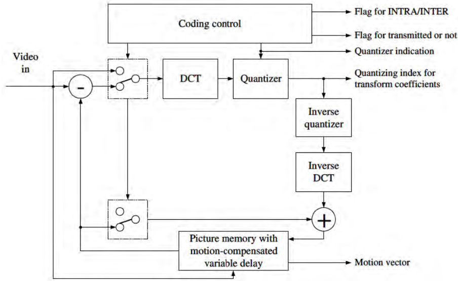
Figure 3.1: H.263 video encoder
