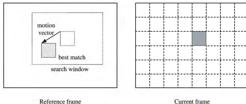
Figure 2.16: Block-matching motion estimation
