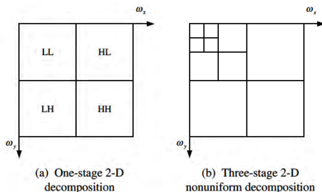
Figure 2.12: Two-dimensional subband decomposition
