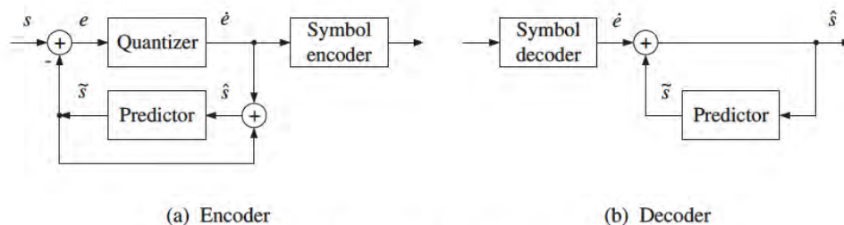
Figure 2.8: Block diagram of a predictive coding system
