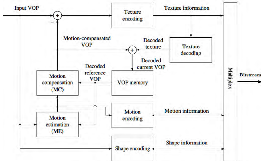
Figure 3.10: An MPEG-4 VOP encoder
