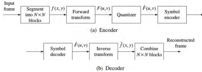
Figure 2.9: Block diagram of a transform coding system
