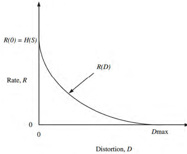
Figure 2.4: Rate-distortion function
