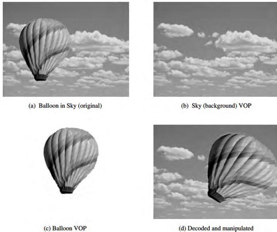
Figure 3.9: Object-based representation, coding, and interaction
