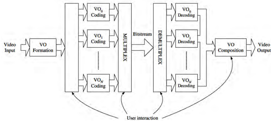
Figure 3.8: An MPEG-4 codec
