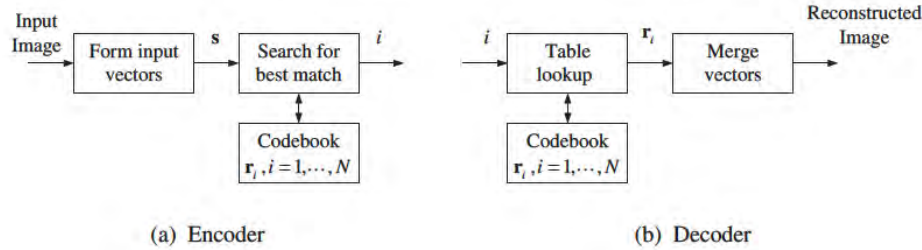
Figure 2.13: A vector quantization system
