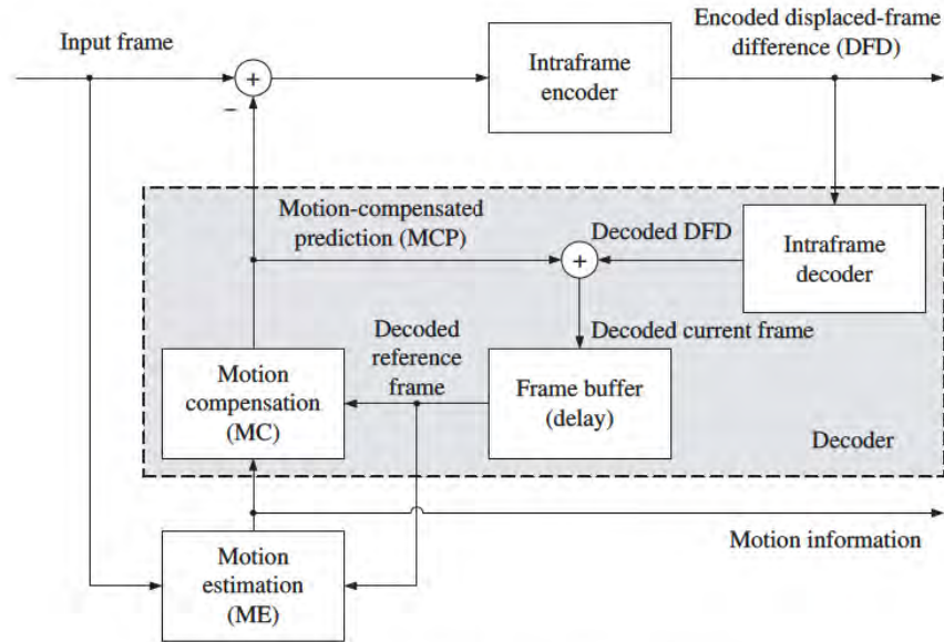
Figure 2.15: Motion-compensated coding system
