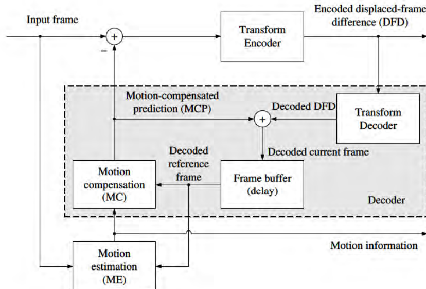
Figure 1.1: Typical video codec
