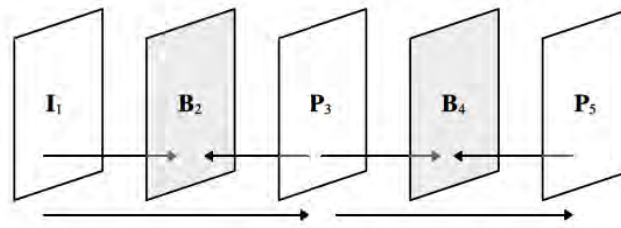
(a) Temporal scalability
