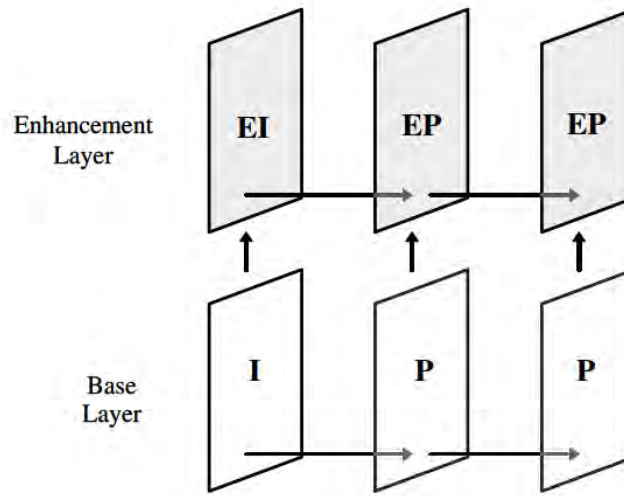
(b) SNR scalability
