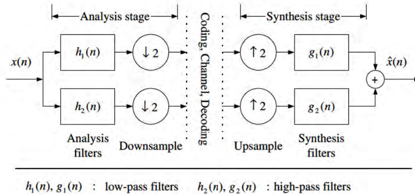
Figure 2.11: A 1-D, two-band subband coding system
