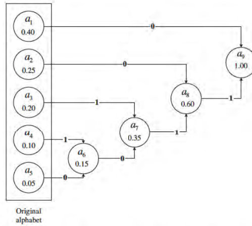
Figure 2.6: Huffman coding example
