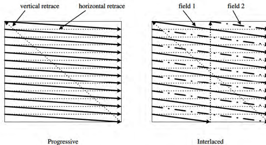
Figure 2.1: Raster scanning methods
