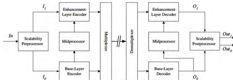
Figure 3.15: MPEG-4 generalized scalability
