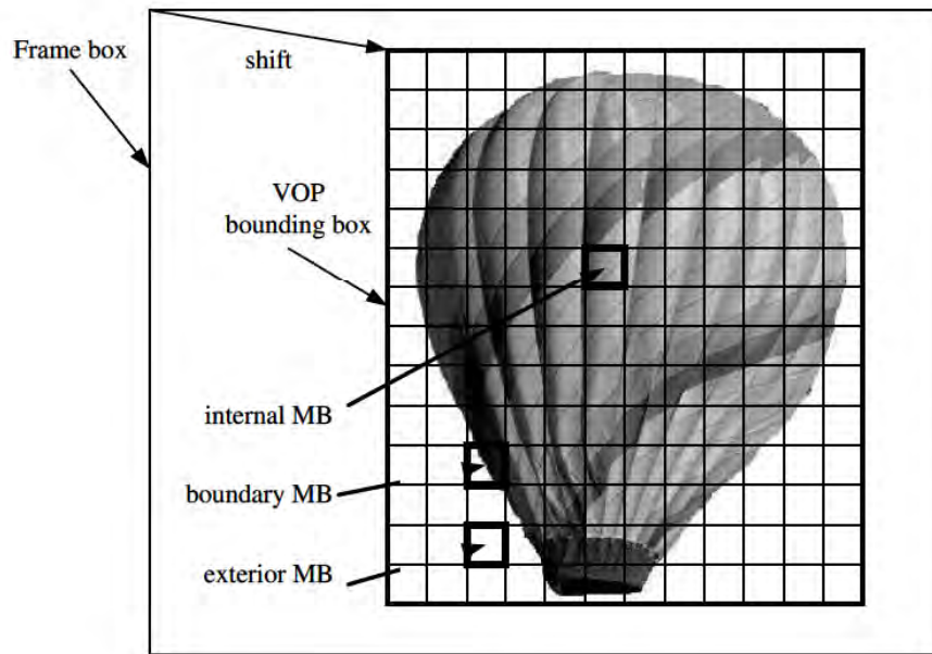
Figure 3.11: The bounding box of the Balloon VOP
