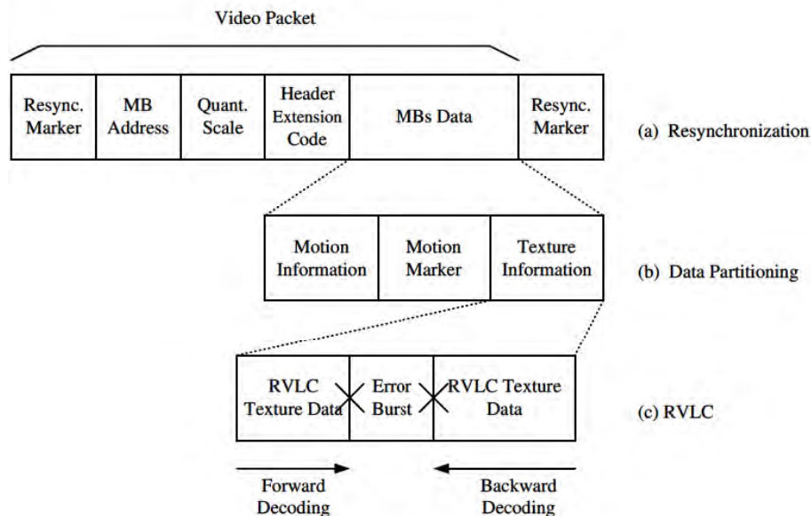
Figure 3.16: MPEG-4 error resilience tools
