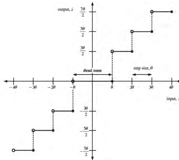
(b) With dead zone
