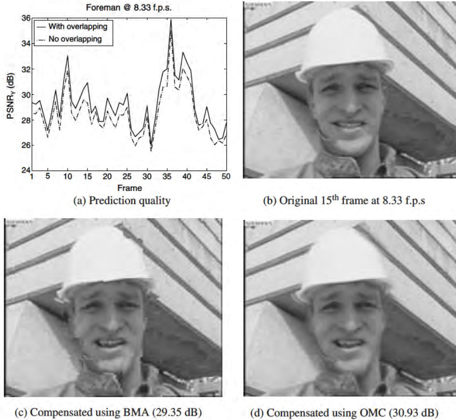
Figure 4.9: Comparison between OMC and BMA
