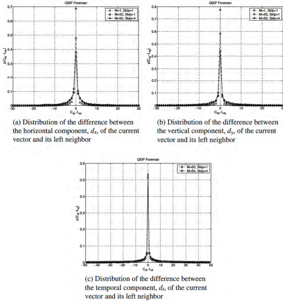
Figure 6.4: Highly correlated long-term memory block-motion field
