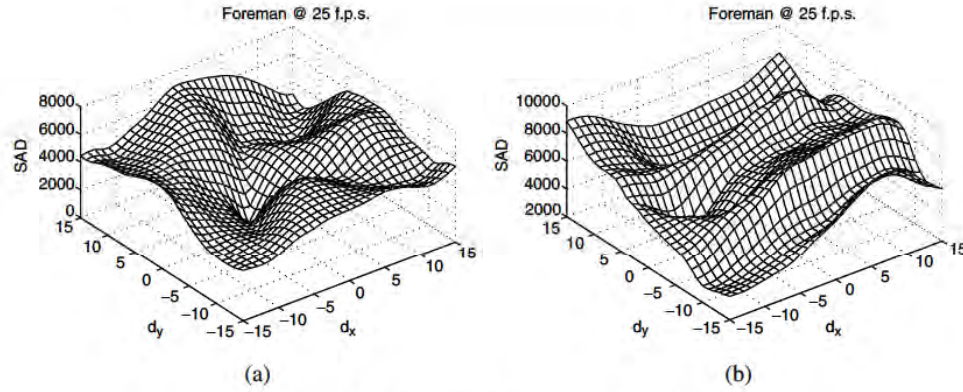
Figure 4.12: Sample multimodal error surfaces
