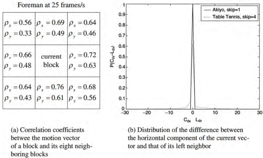
Figure 4.11: Highly correlated block-motion fields
