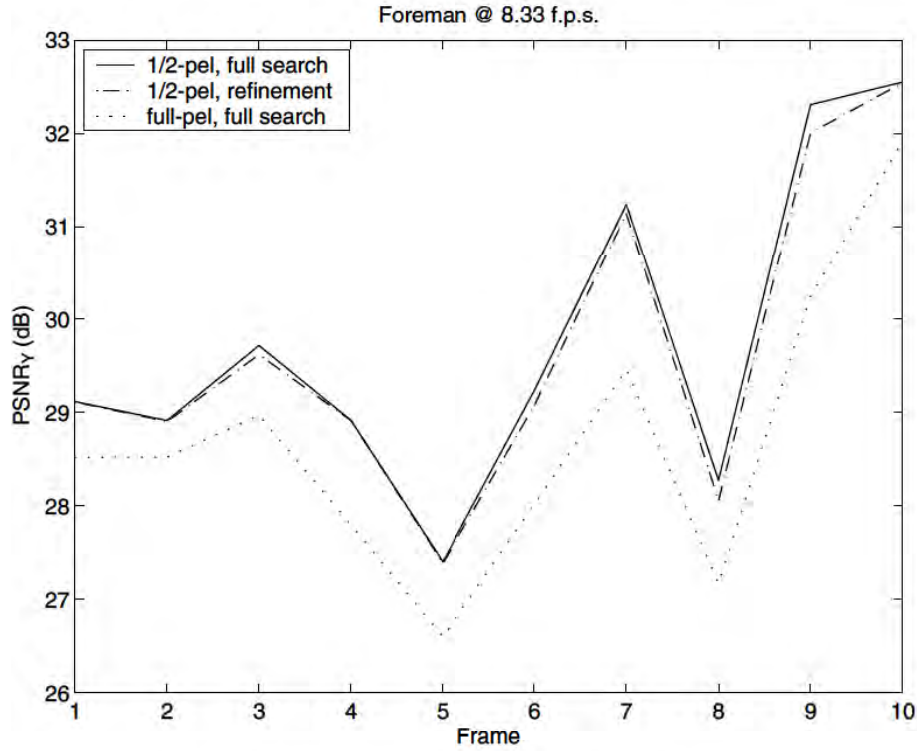
Figure 4.6: Performance of the BMA with subpel accuracy
