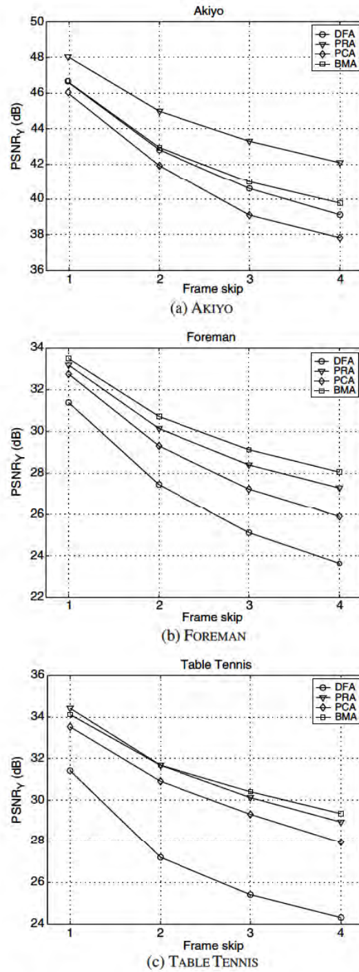
Figure 4.13: Prediction quality of different motion estimation algorithms
