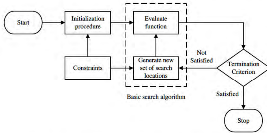
Figure 8.1: Basic building blocks of constrained optimization methods
