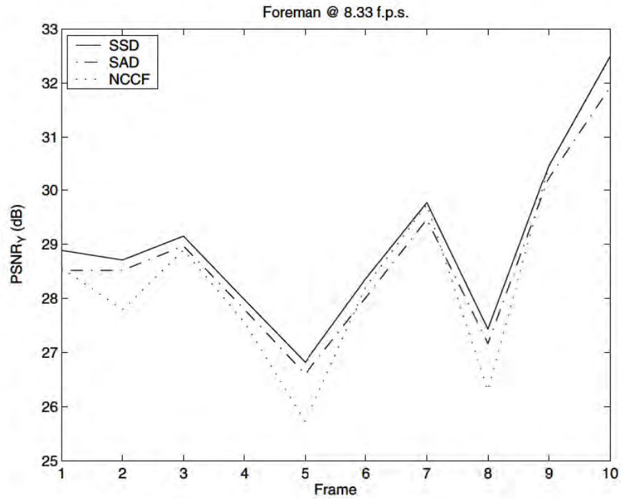
Figure 4.3: Reconstruction quality of SSD, SAD, and NCCF
