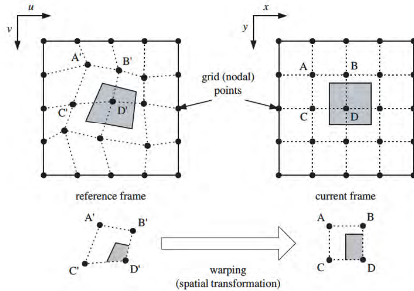
Figure 5.1: Warping-based motion estimation and compensation
