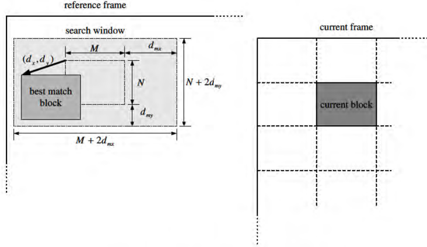
Figure 4.2: Block-matching motion estimation
