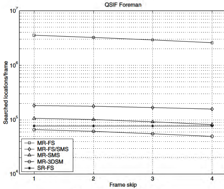
Figure 8.11: Comparison between different block-matching algorithms when applied to QSIF FOREMAN with a multiframe memory of M = 50 frames
