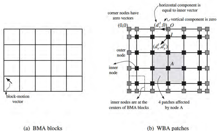
Figure-5.3:- BMA-blocks-and-WBA-patches-
