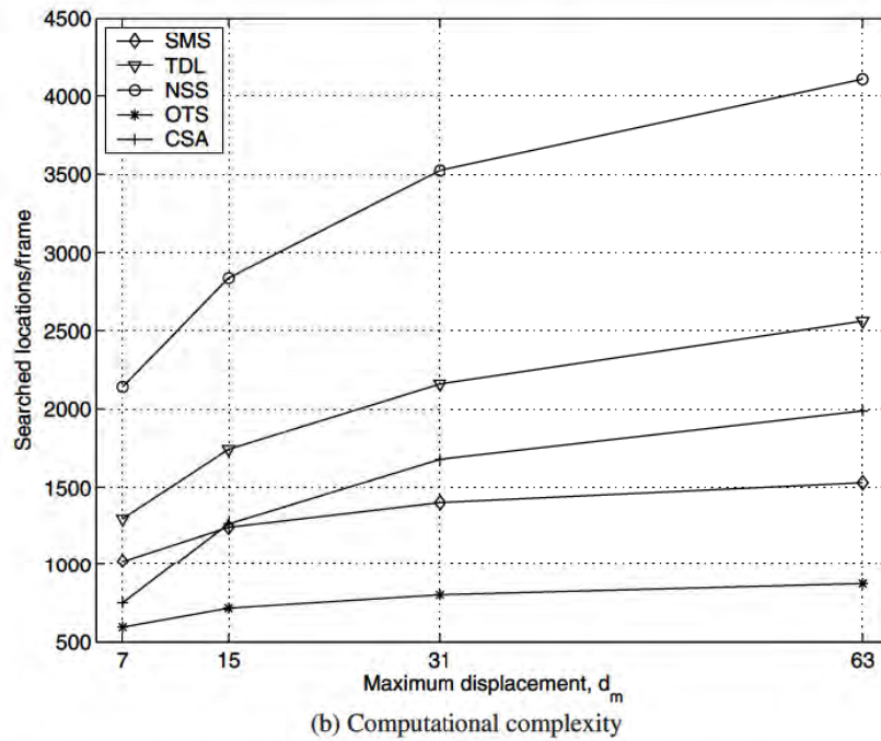
Figure 8.6: Comparison between different block-matching algorithms when applied to QSIF FOREMAN with maximum displacements of 7, 15, 31, and 63 and corresponding frame rates of 25, 12.5, 8.33, and 6.25 frames/s, respectively
