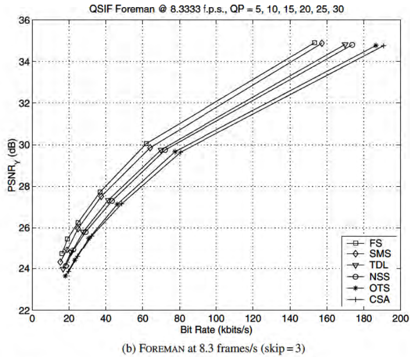
Figure 8.7: R-D performance of different block-matching algorithms when applied to QSIF FOREMAN
