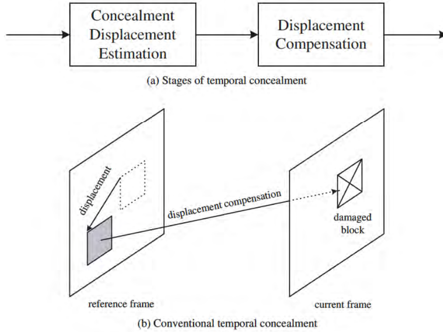
Figure 9.8: Temporal error concealment
