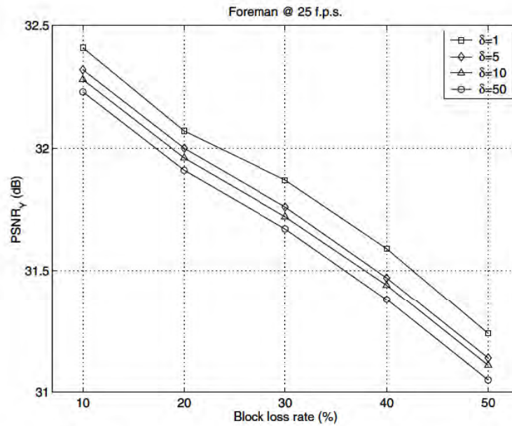
Figure 10.4: Performance of BM-MFI when applied to QSIF FOREMAN at 25 frames/s with different multihypothesis weights. PSNRs are for damaged blocks only
