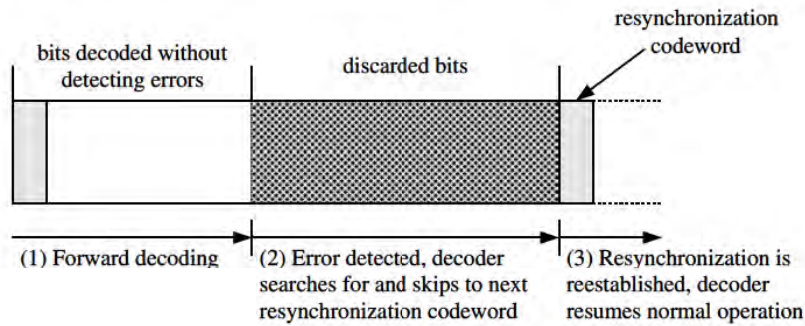
(a) Resynchronization with normal VLC coding
