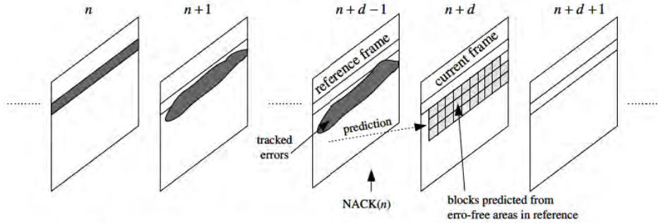
(c) Restricted prediction based on error tracking and feedback information
