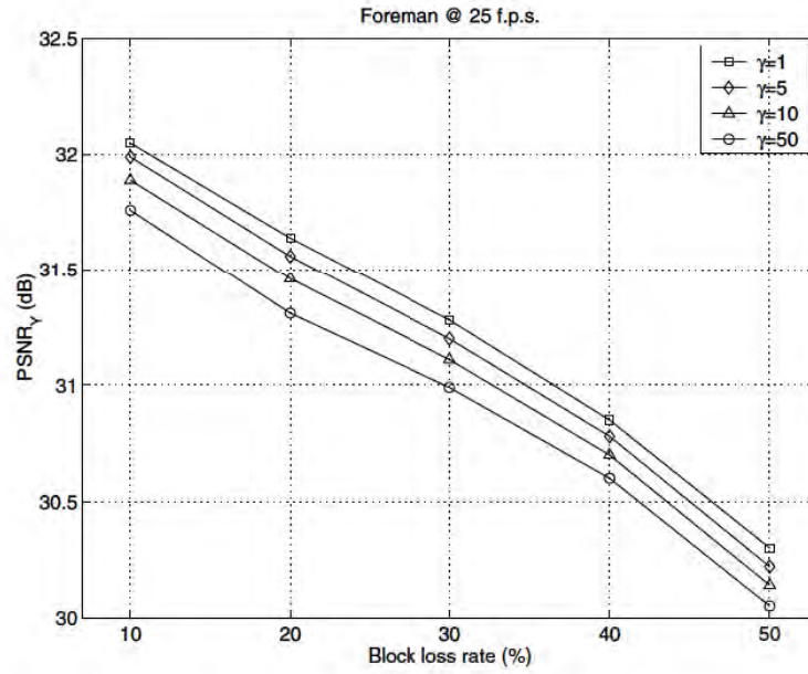
Figure 10.3: Performance of MFI when applied to QSIF FOREMAN at 25 frames/s with different interpolation kernels. PSNRs are for damaged blocks only
