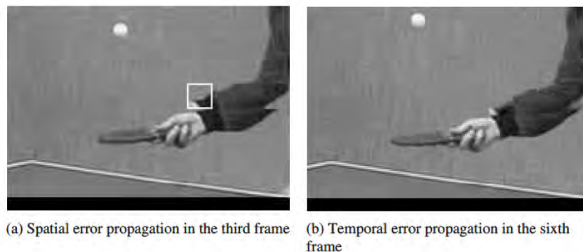
Figure 9.2: Spatial and temporal error propagation due to a single-bit error in QSIF TABLE TENNIS H.263 encoded at 10 frames/s (46 kbits/s)
