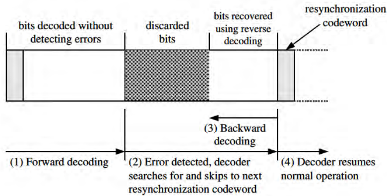
(b) Resynchronization with reversible VLC (RVLC) coding
