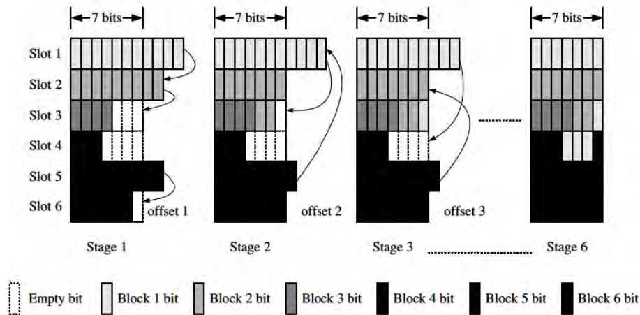
Figure 9.5: Example of the EREC algorithm
