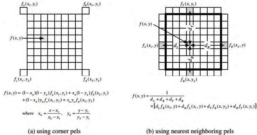
Figure 9.7: Error concealment using spatial interpolation
