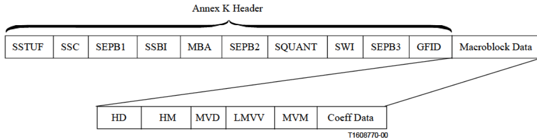
Figure V.1/H.263 – Data partitioning syntax
