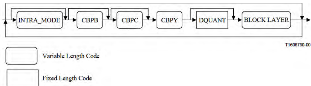
Figure V.3/H.263 – Coefficient Data syntax
