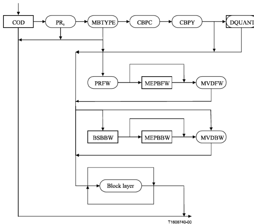
Figure U.7/H.263 – Structure of EP- and B-picture macroblock layer for the ERPS mode
