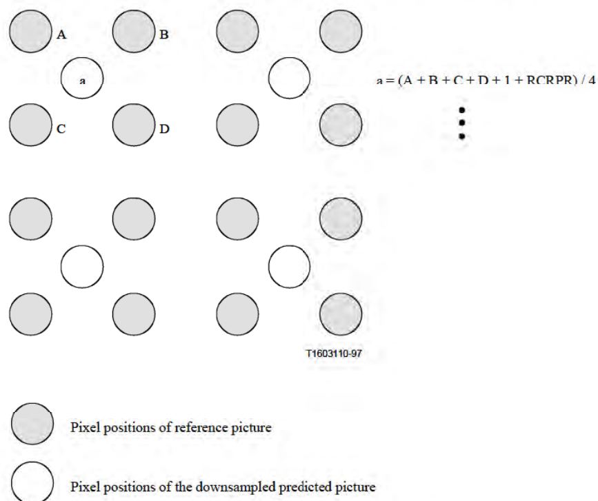
Figure P.6/H.263 – Factor-of-4 downsampling
