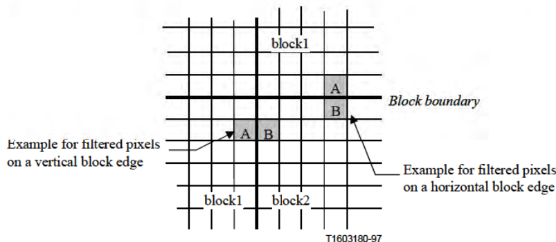
Figure Q.10/H.263 – Default block boundary filter
