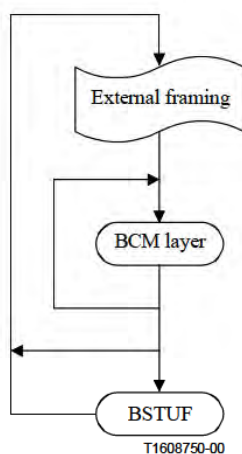
Figure U.8/H.263 – Structure of BCM separate logical channel layer for ERPS mode
