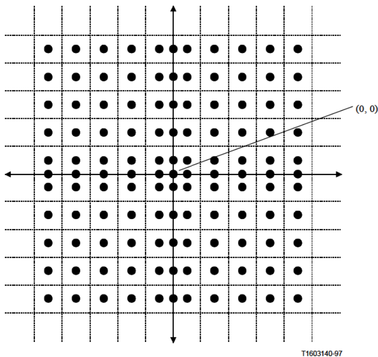
Figure Q.3/H.263 – Reconstruction of motion vector
