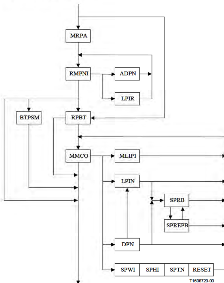
Figure U.5/H.263 – Structure of the ERPS layer
