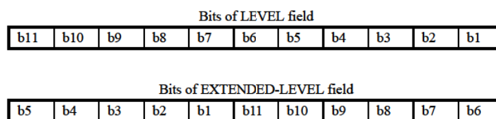
Figure T.1/H.263 – Cyclic rotation of coefficient representation
