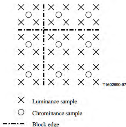
Figure 2/H.263 – Positioning of luminance and chrominance samples
