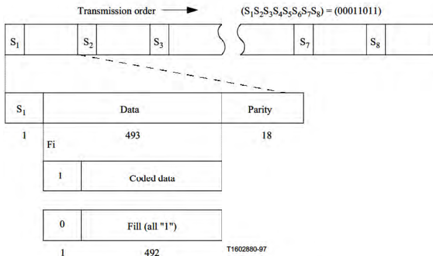
Figure H.1/H.263 – Error correcting frame
