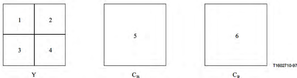
Figure 5/H.263 – Arrangement of blocks in a macroblock
