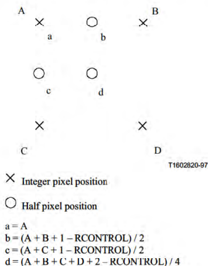
Figure 13/H.263 – Half-pixel prediction by bilinear interpolation
