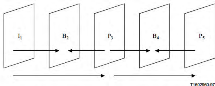
Figure O.1/H.263 – Illustration of B-picture prediction dependencies
