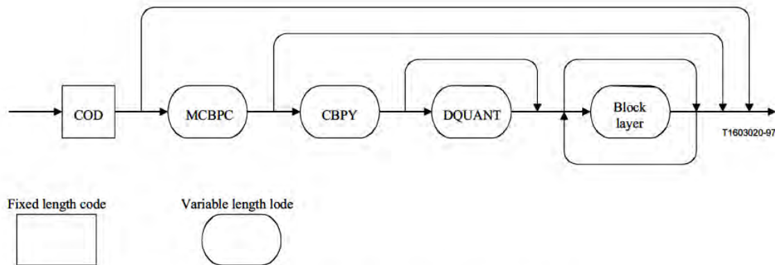
Figure O.7/H.263 – Macroblock syntax for EI-pictures
