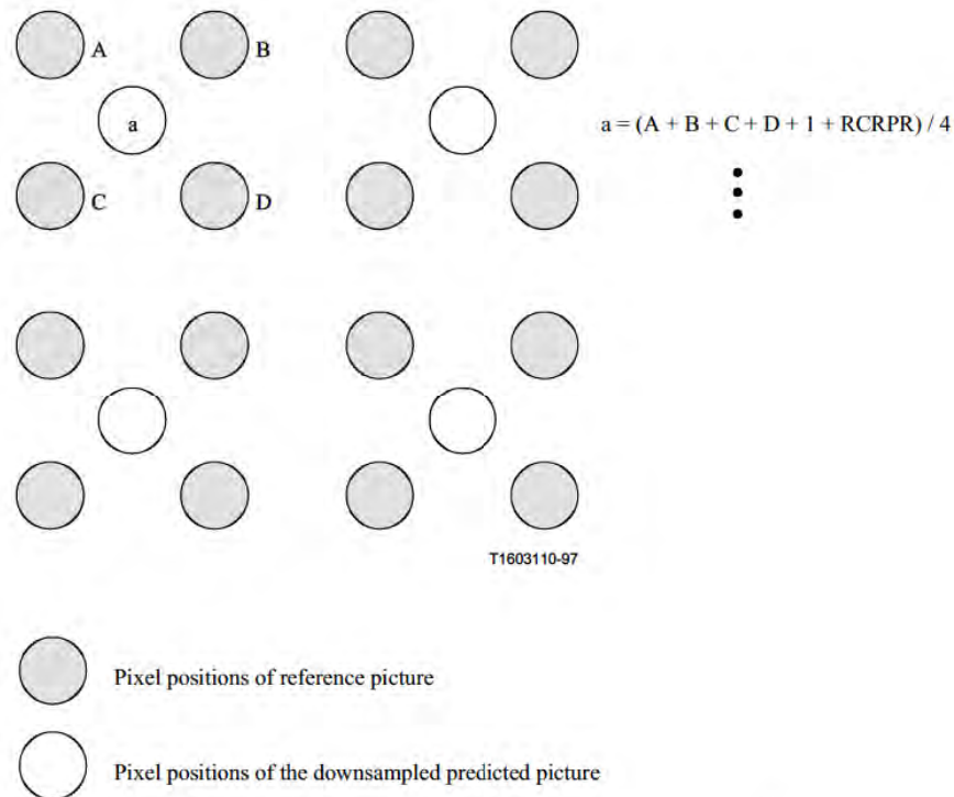
Figure P.6/H.263 – Factor-of-4 downsampling
