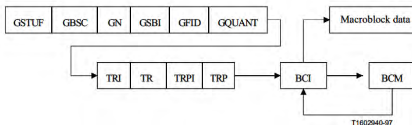
Figure N.2/H.263 – Structure of GOB layer for NEWPRED
