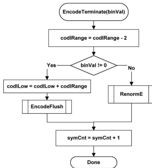
Figure 9-11 – Flowchart of encoding a decision before termination
