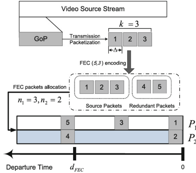
Fig. 3 Illustration of the scheduling process of the proposed loss tolerant bandwidth aggregation for FEC data packets
