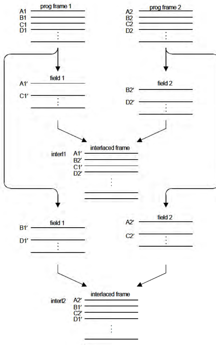
Figure D.3 – Progressive to two-interlace conversion
