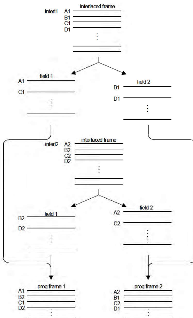
Figure D.4 – Two-interlace to progressive conversion
