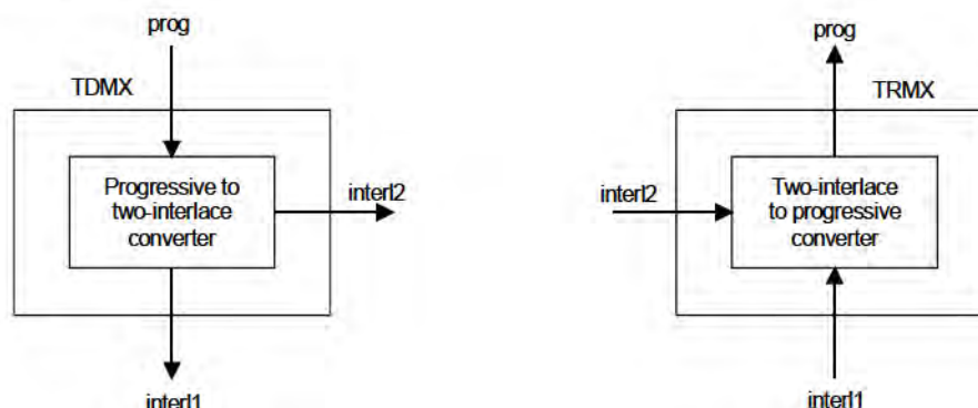
Figure D.5 – Temporal demultiplexer and remultiplexer for progressive – Interface-to-interface temporal scalability
