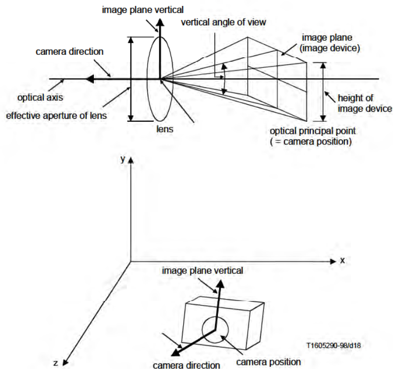
Figure 6-17 -- Camera parameters
