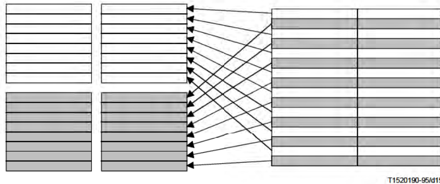
Figure 6-14 – Luminance macroblock structure in field DCT coding
