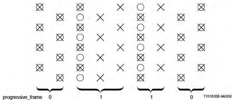
Figure 7-22 – progressive_sequence = 0 with 4:2:2 or 4:4:4 chrominance
