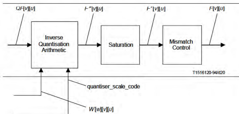
Figure 7-4 – Inverse quantisation process
