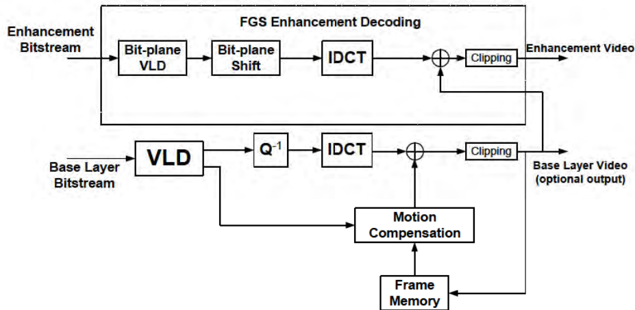
Figure 0-5 — A Basic FGS Decoder Structure
