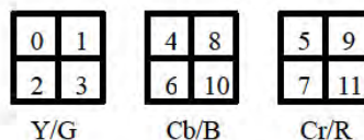
Figure 6-10 — 4:4:4 Macroblock structure
