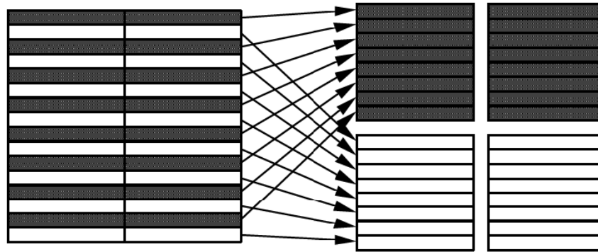
Figure 6-12 — Luminance macroblock structure in field DCT coding
