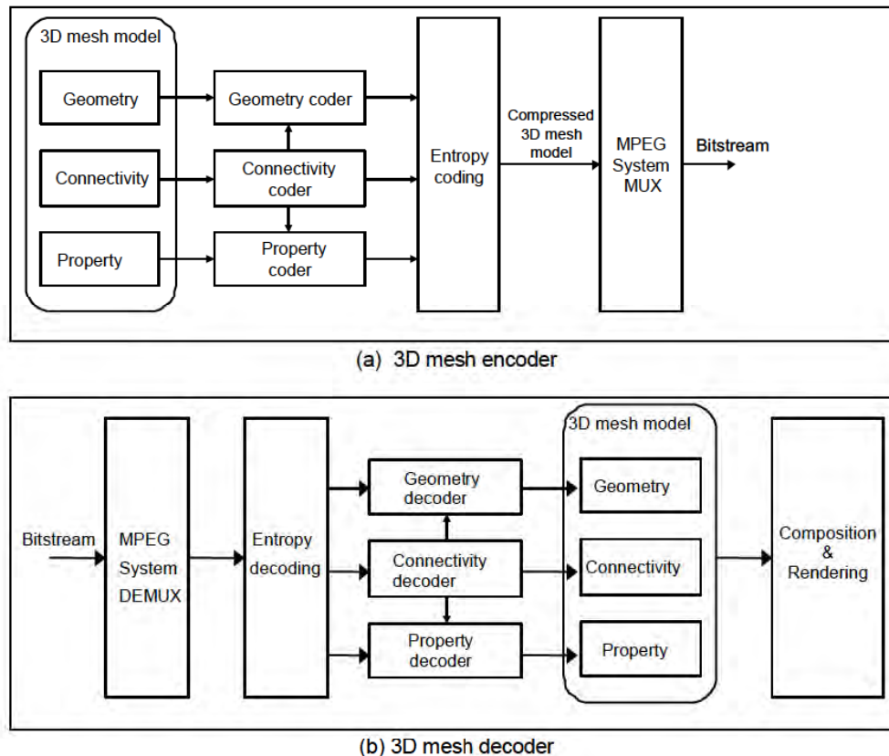
Figure 0-4 — General block diagram of the 3D mesh compression system
