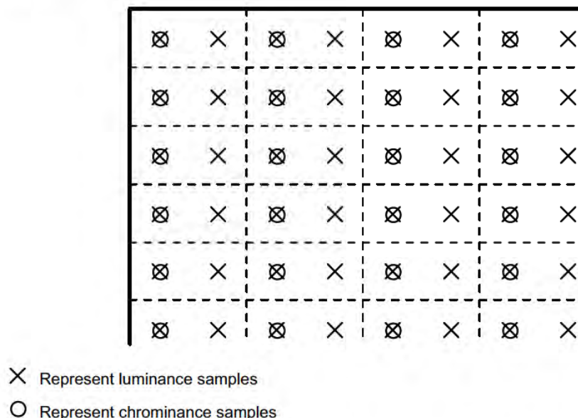
Figure 6-5 — The position of luminance and chrominance samples. 4:2:2 data.
