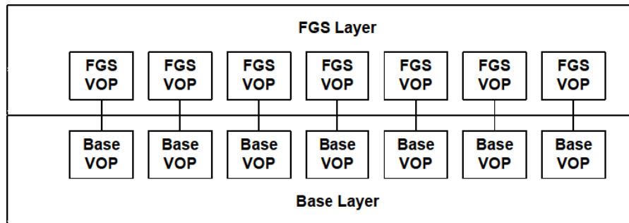
Figure 0-6 — Basic FGS Enhancement Structure
