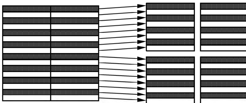
Figure 6-11 — Luminance macroblock structure in frame DCT coding
