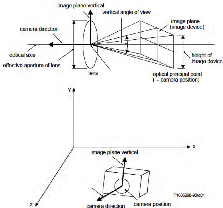
Figure 6-23 — Camera parameters
