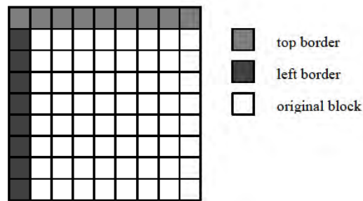
Figure 7-23 — Extension of border pixels
