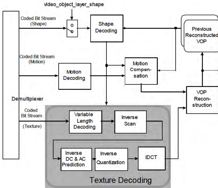
Figure 7-2 — Simplified Video Decoding Process
