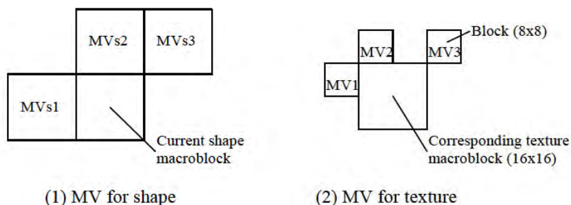
Figure 7-12 — Candidates for MVPs
