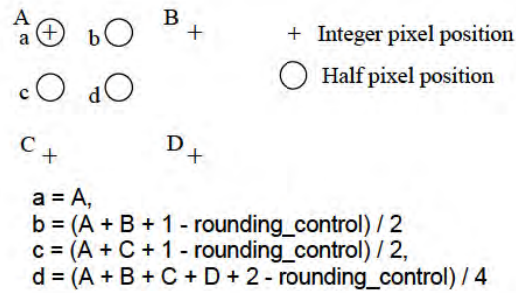
Figure 7-29 — Interpolation scheme for half sample search
