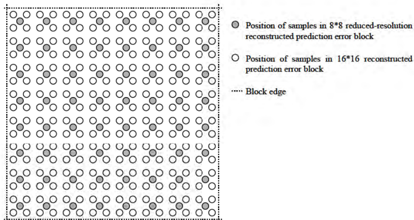
Figure 7-8 — Positioning of samples in 8×8 reduced-resolution reconstructed prediction error block and 16×16 reconstructed prediction error block
