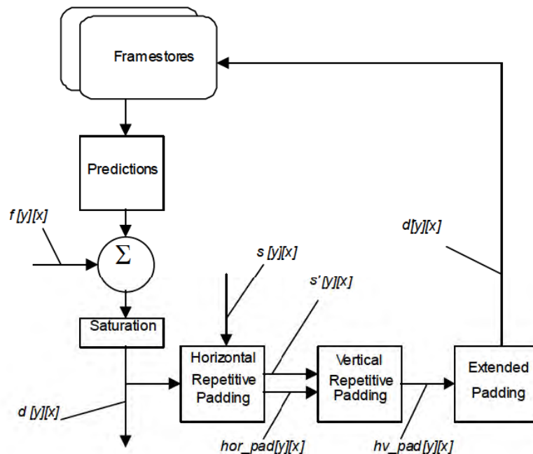
Figure 7-27 — Simplified padding process
