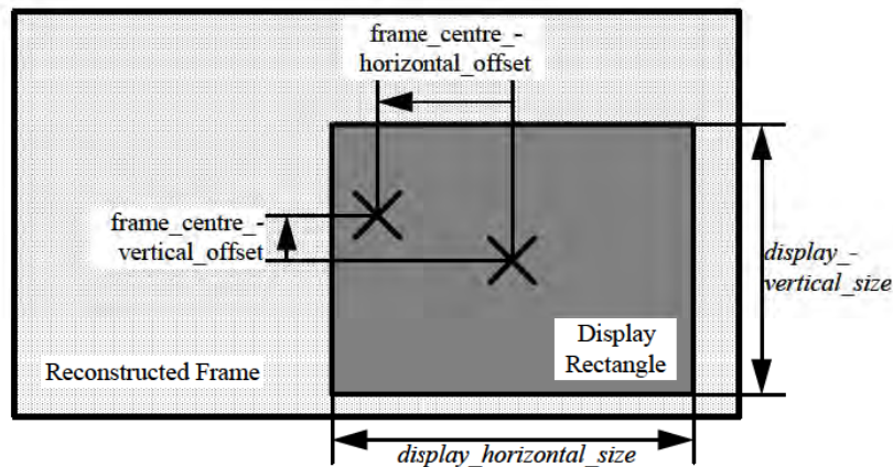
Figure 6-22 — Frame centre offset parameters
