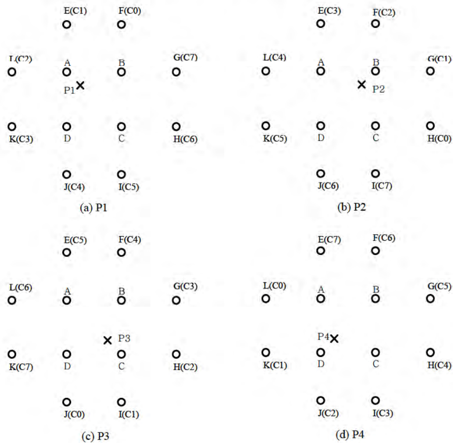
Figure 7-17 — Interpolation filter and interpolation construction
