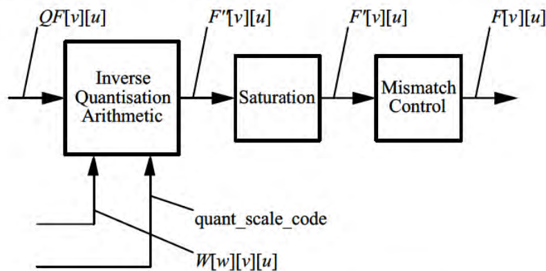
Figure 7-7 — Inverse quantisation process
