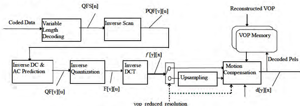
Figure 7-3 — Video Texture Decoding Process
