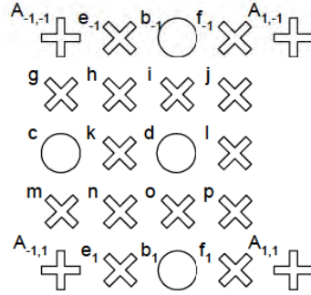
Figure 7-32 — Quarter sample interpolation in quarter sample mode (FIR and bilinear filter)
