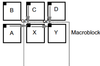
Figure 7-5 — Previous neighboring blocks used in DC prediction
