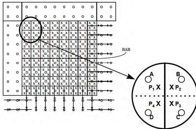
Figure 7-16 — Upsampling
