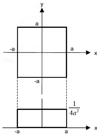
Figure 6-24 — Defocusing filter
