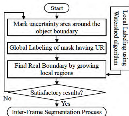
Figure F.13 — Intra-Frame Segmentation Process
