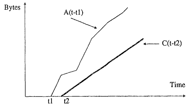
Fig.4 Average arriving rate is larger than the output rate, buffer requirement becomes larger and larger with time
