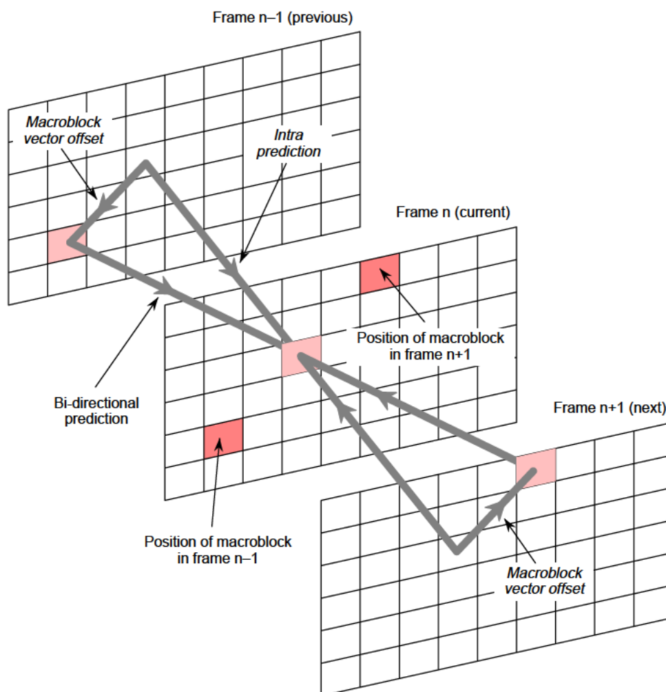
Figure 10 Motion-compensated bi-directional prediction.
