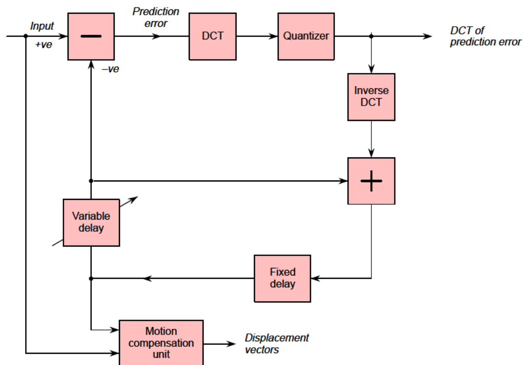
Figure 11 Motion-compensated interframe prediction DCT.
