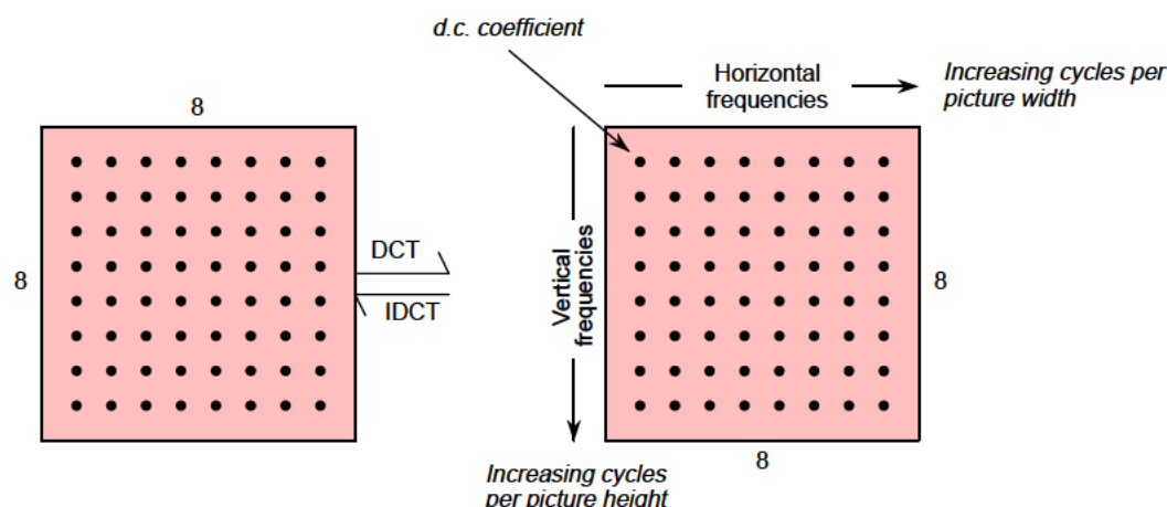
Figure 3 DCT transform pairs.
