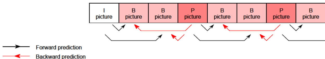
Figure 13 MPEG picture types.
