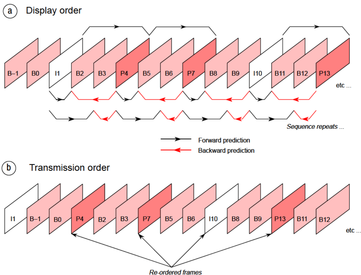
Figure 14 Example Group of Pictures (GOP).
