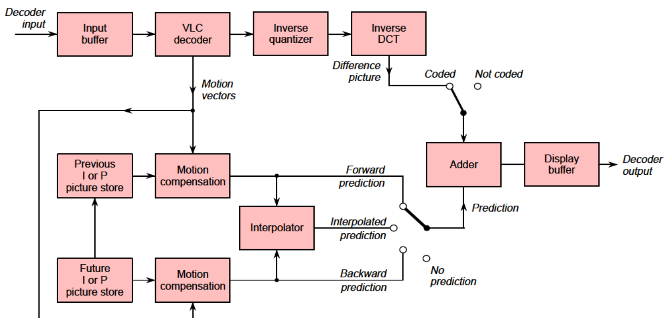
Figure 12 Decoding a "B" macroblock.
