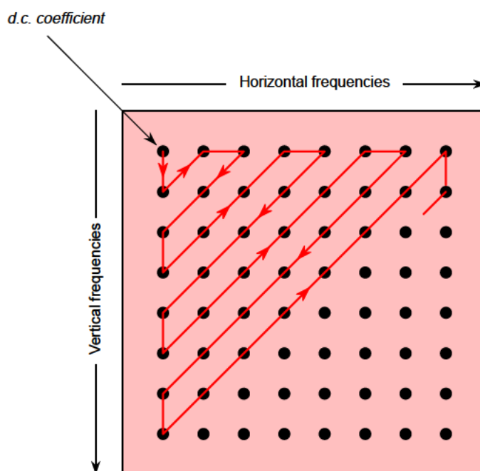
Figure 4 Scanning of DCT blocks and run-length coding with variable-length codes (Entropy coding).
