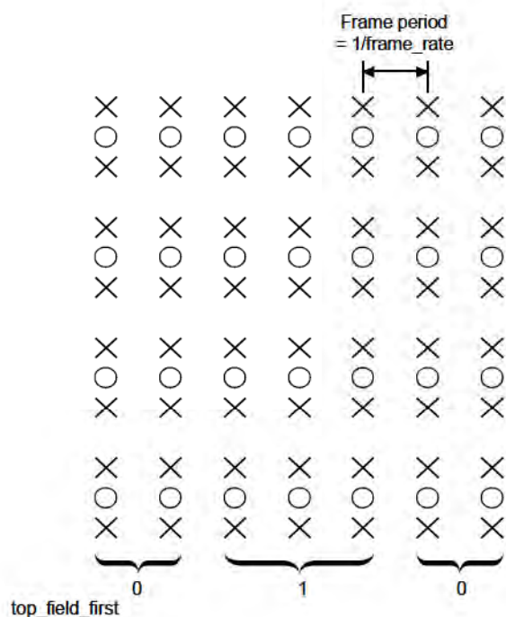
Figure 7-19 – progressive_sequence == '1'; repeat_first_field == '1'
