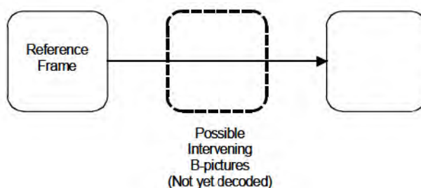
Figure 7-10 – Frame-prediction for I-pictures and P-pictures
