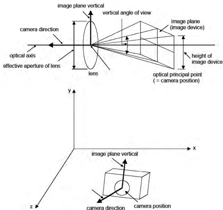
Figure 6-17 – Camera parameters
