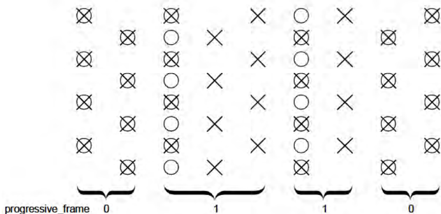
Figure 7-22 – progressive_sequence = 0 with 4:2:2 or 4:4:4 chrominance
