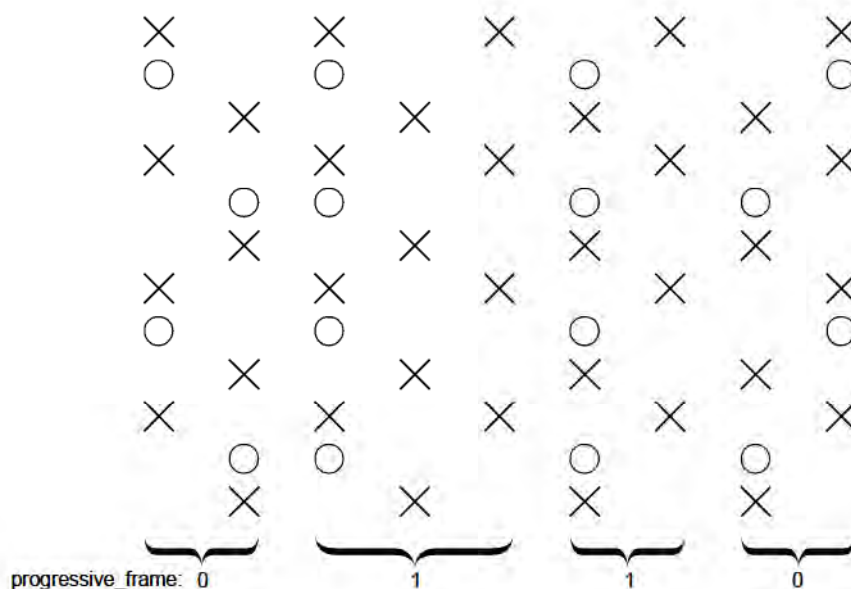
Figure 7-21 – progressive_sequence = 0 with 4:2:0 chrominance
