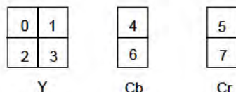
Figure 6-11 – 4:2:2 Macroblock structure
