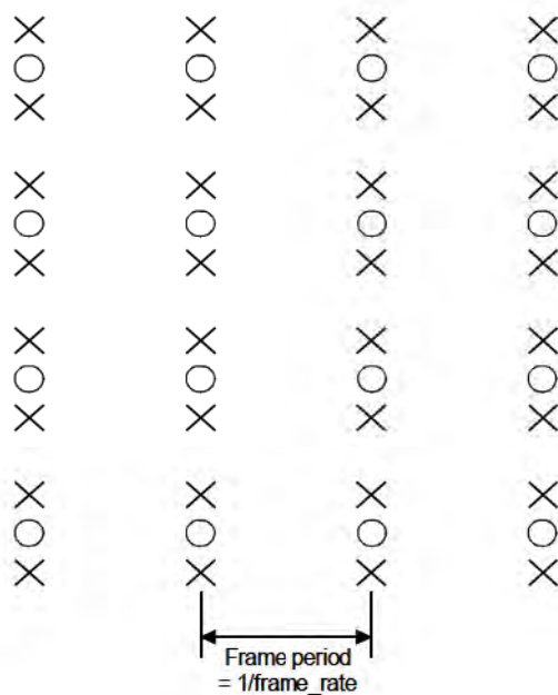
Figure 7-18 – progressive_sequence == 1
