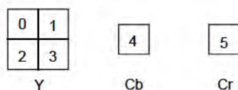
Figure 6-10 – 4:2:0 Macroblock structure
