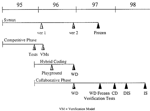
Fig. 6 MPEG4 workplan.
