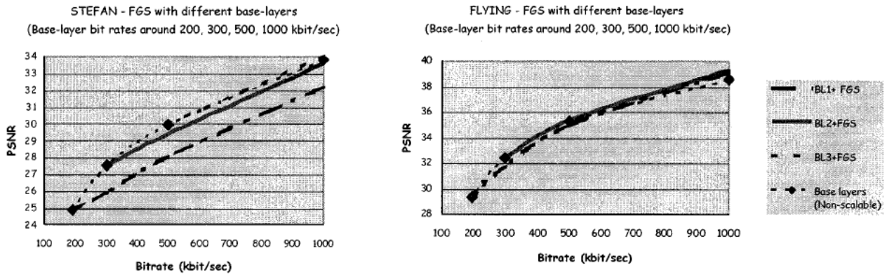
Fig. 8. FGS performance in comparison with multiple non-scalable streams' (ideal) case. The left figure shows the results for a sequence that exhibits a high-degree of temporal correlation among successive frames. For this type of sequences, FGS pay penalty in performance due to the absence of motion compensation within the enhancement-layer. The right figure shows the performance for a sequence with very-high motion and a large number of scene cuts. For this type of sequences, FGS performance is either similar to or even slightly better than the ideal non-scalable case.
