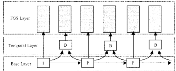
Fig. 16. Multilayer FGS-temporal scalability structure.
