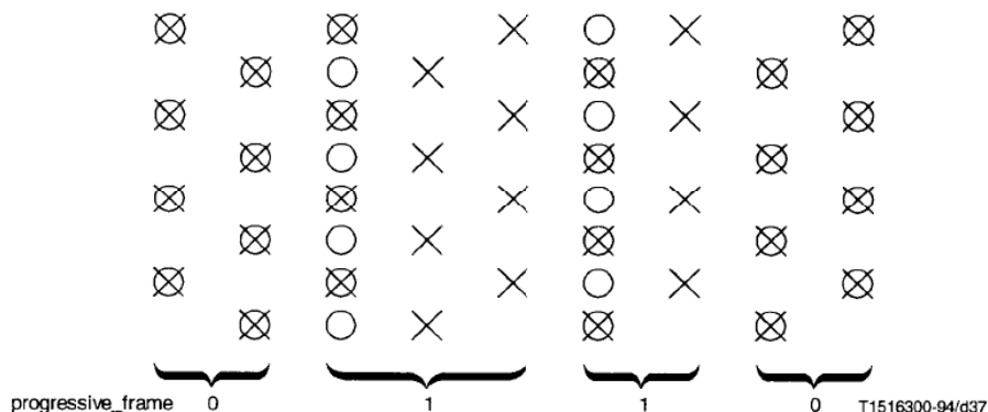
Figure 7-22 – progressive_sequence == 0 with 4:2:2 or 4:4:4 chrominance
