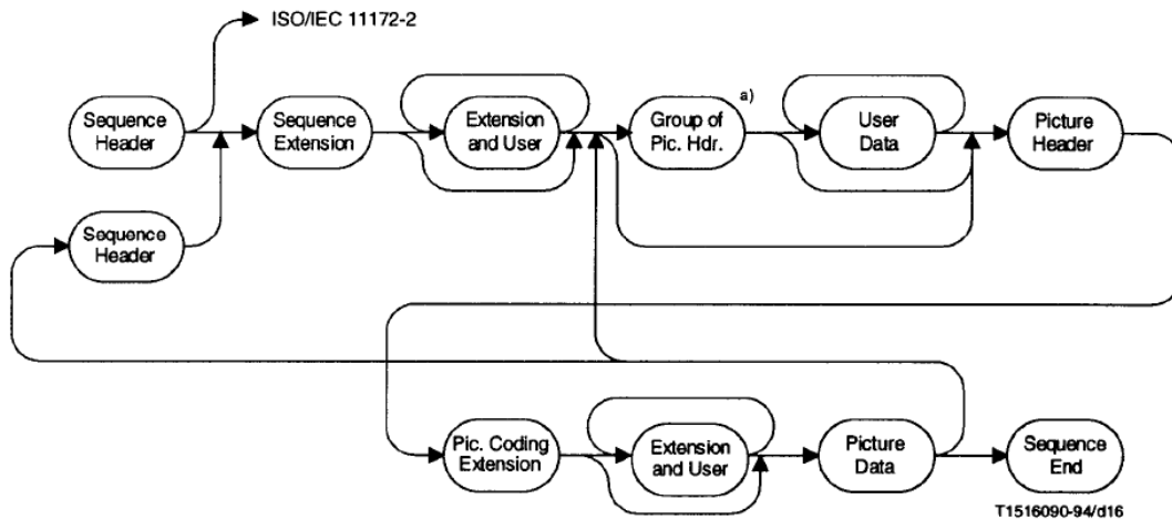
Figure 6-15 – High level bitstream organisation
