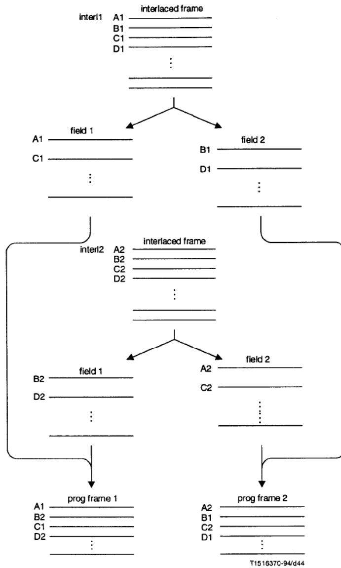
Figure D.4 – Two interlace to progressive conversion
