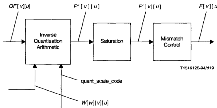
Figure 7-4 – Inverse quantisation process
