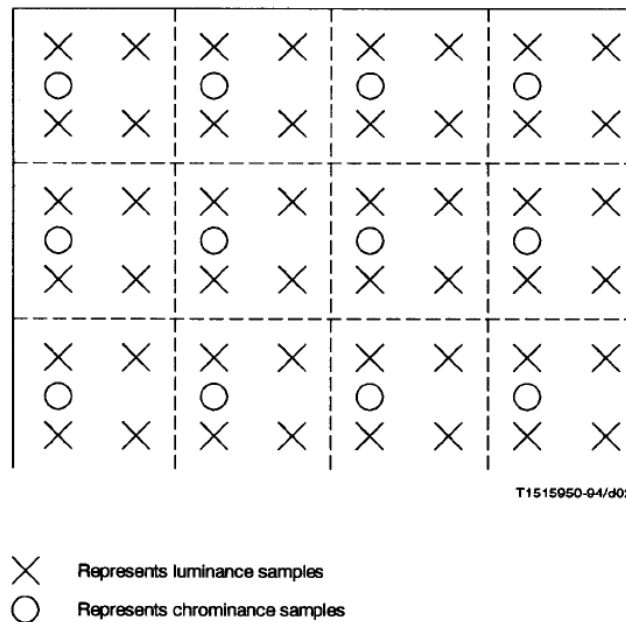
Figure 6-1 – The position of luminance and chrominance samples – 4:2:0 data
