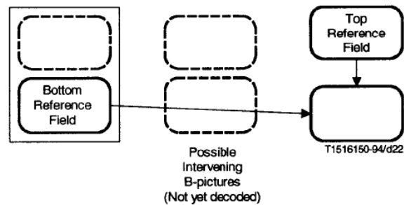
Figure 7-7 – Prediction of the second field-picture when it is the bottom field
