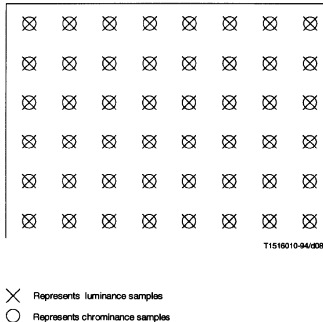
Figure 6-7 – The position of luminance and chrominance samples – 4:4:4 data
