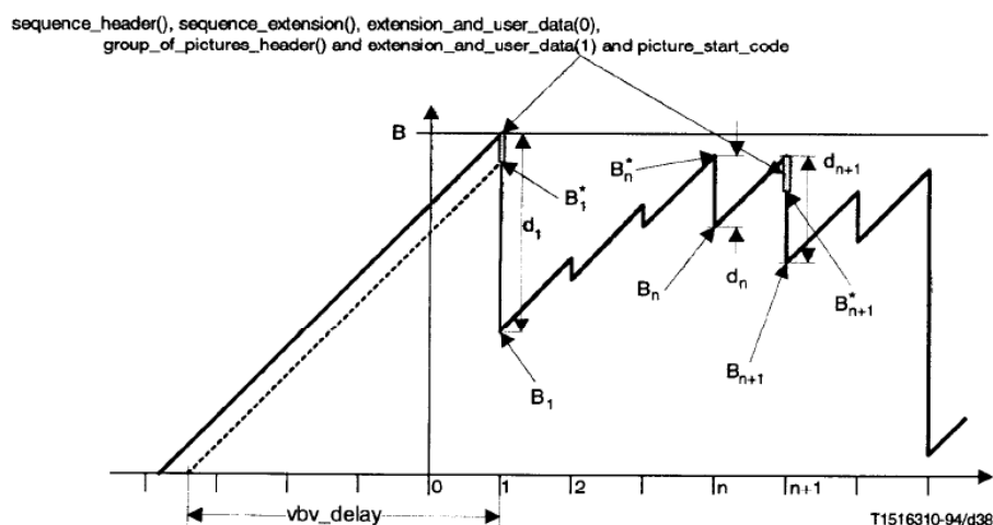
Figure C.1 – VBV Buffer Occupancy – Constant bit-rate operation
