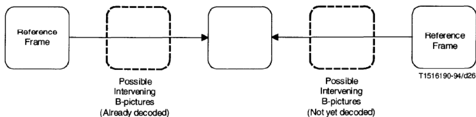
Figure 7-11 – Frame-prediction for B-pictures
