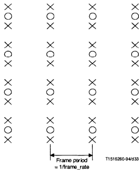
Figure 7-18 – progressive_sequence == 1
