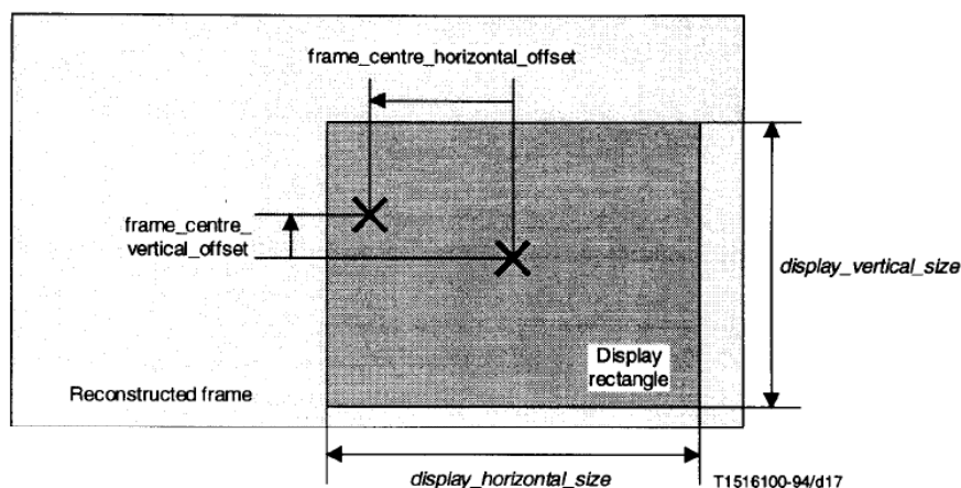
Figure 6-16 – Frame centre offset parameters
