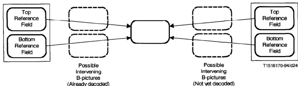
Figure 7-9 – Field-prediction of B-field pictures or B-frame pictures
