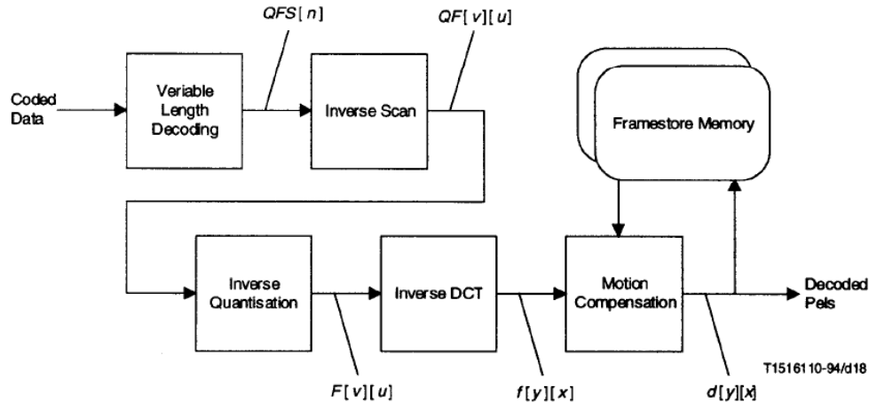
Figure 7-1 – Simplified Video Decoding Process
