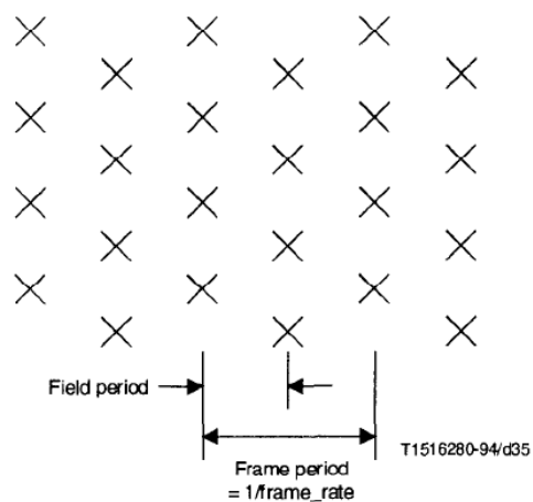
Figure 7-20 – progressive_sequence == 0
