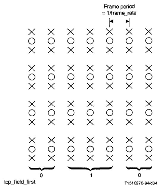
Figure 7-19 – progressive_sequence == 1, repeat_first_field = 1
