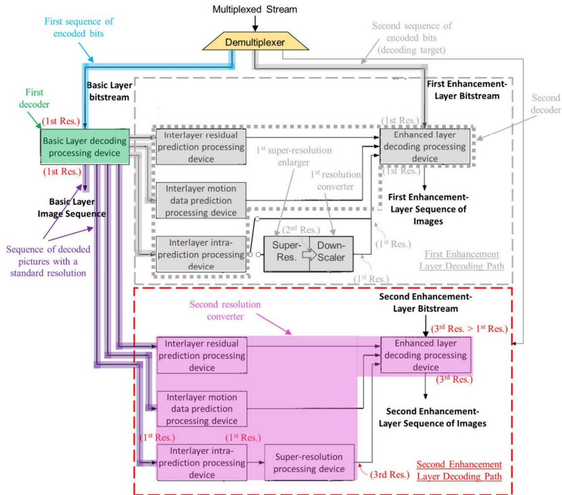
Illustration of Phek-Segall-Martins-He Combination
