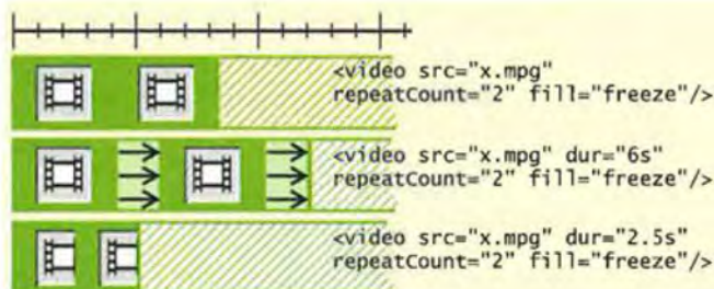
Figure 7-4. SMIL durations.
