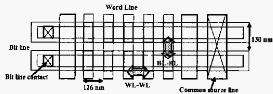
Fig. 1. Schematic diagram of the cell layout and its dimension of the 63nm cell arrays. WL-WL and BL-BL directions are indicated.
