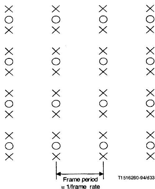
Figure 7-18 – progressive_sequence == 1
