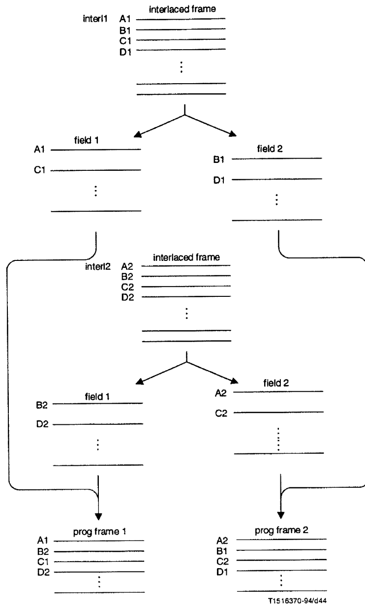
Figure D.4 – Two interlace to progressive conversion
