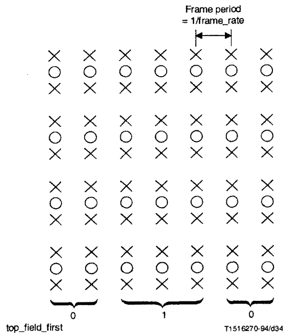
Figure 7-19 – progressive_sequence == 1 , repeat_first_field == 1
