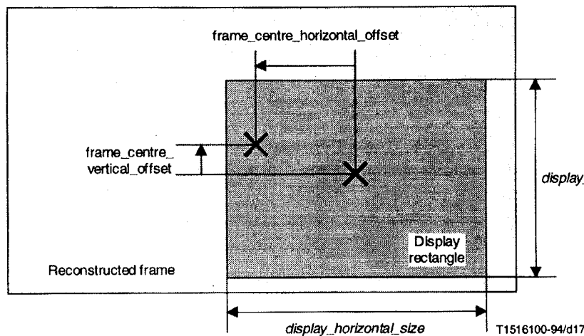
Figure 6-16 – Frame centre offset parameters
