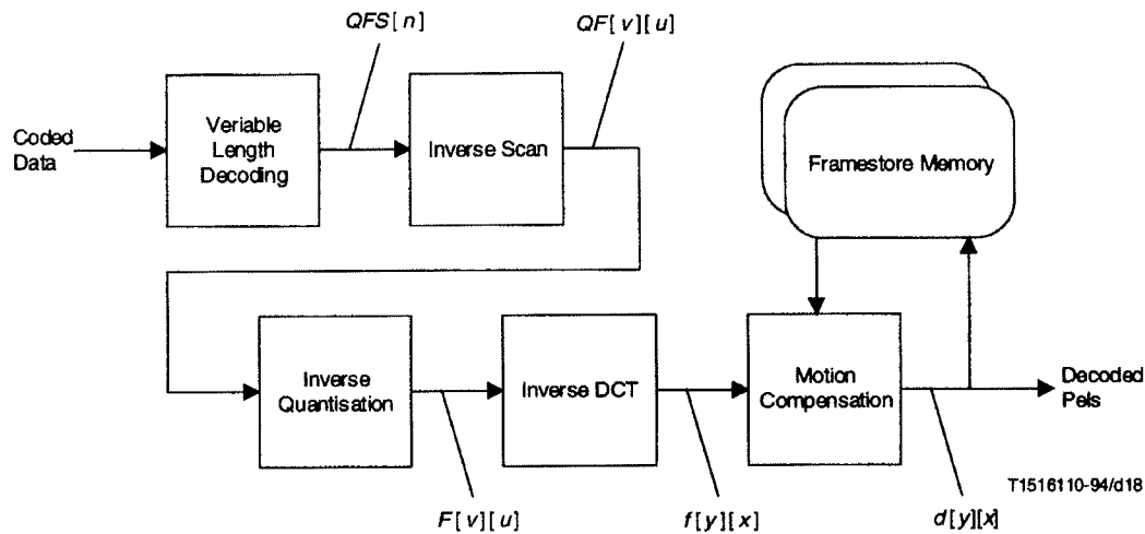
Figure 7-1 – Simplified Video Decoding Process
