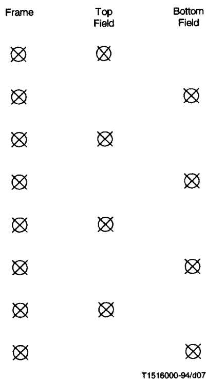
Figure 6-6 – Vertical positions of samples with 4:2:2 and 4:4:4 data
