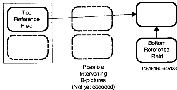
Figure 7-8 – Prediction of the second field-picture when it is the top field
