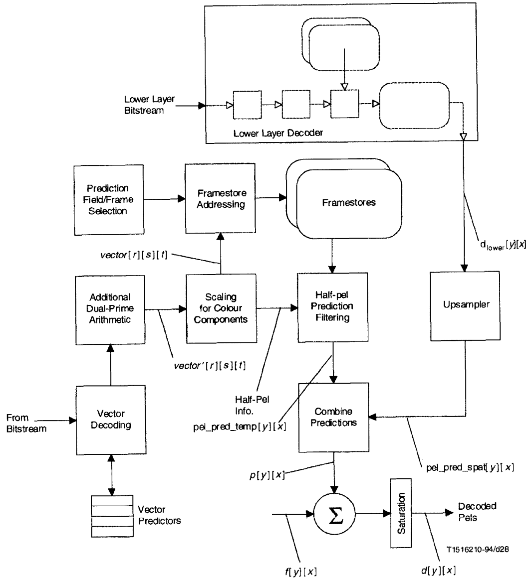
Figure 7-13 – Simplified motion compensation process for spatial scalability
