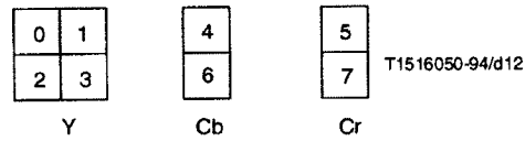
Figure 6-11 – 4:2:2 Macroblock structure
