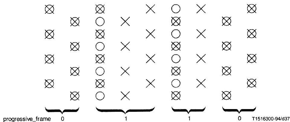
Figure 7-21 – progressive_sequence == 0 with 4:2:0 chrominance
