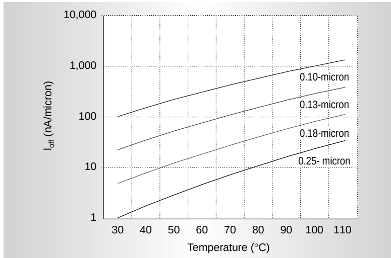
Figure 10. Projected I_{off} .
