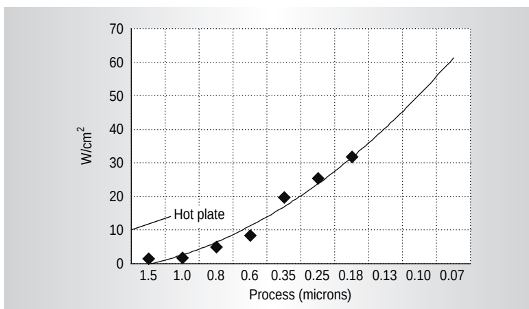
Figure 12. Chip power density.
