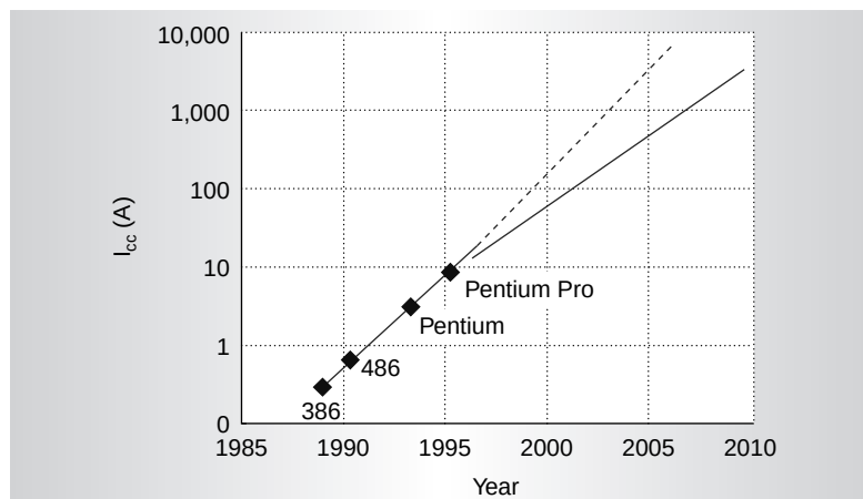
Figure 9. Supply current projections.
