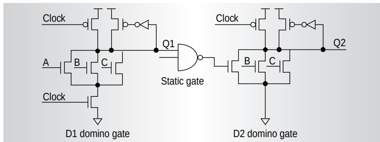
Figure 11. Domino circuit.
