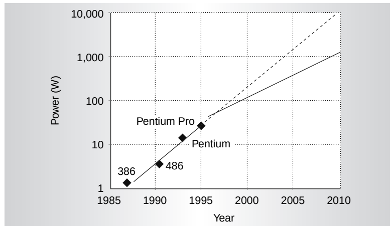
Figure 8. Power dissipation projections.
