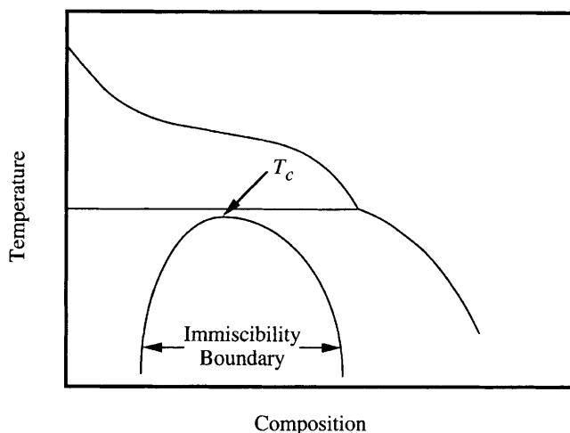
Figure 4.6 Idealized phase diagram for a binary system exhibiting metastable immiscibility
