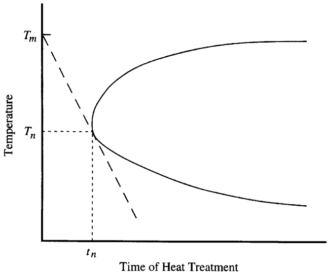
Figure 2.2 A time–temperature–transformation curve for a glass forming melt
