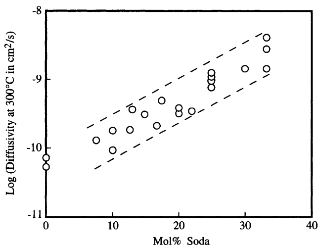
Figure 8.1 Effect of sodium concentration on the diffusivity at 300 °C of sodium ions in sodium silicate glasses
