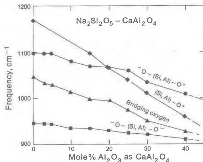
Fig. 7. Frequency change of important Raman bands in the system \text{Na}_2\text{Si}_2\text{O}_5\text{--CaAl}_2\text{O}_4 as a function of Al content (mole % \text{Al}_2\text{O}_3 on the basis of 5 oxygens).
