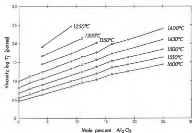
Fig. 2. Plot of \log \eta vs. mole% \text{Al}_2\text{O}_3 . Isotherms at 50°C intervals between 1250–1600°C.
