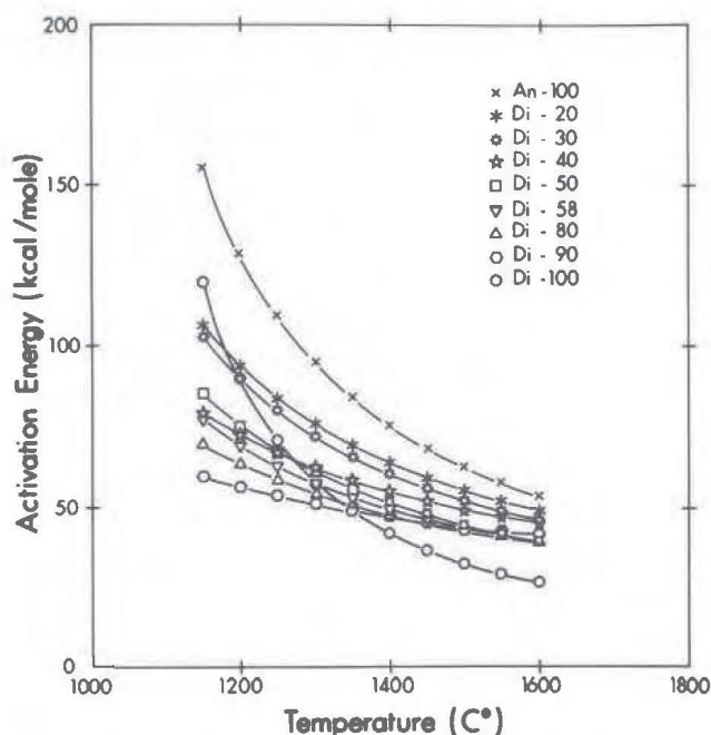
Fig. 4. Activation energy for viscous flow vs. temperature.
