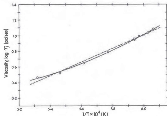
Fig. 3. Plot of \log \eta vs. 1/T for diopside melt. Broken line is Arrhenius fit and solid line is Fulcher fit. Circles are experimental data points. Additional data points for diopside at 1410°C (0.942, 0.959), 1395°C (1.003) and 1385°C (1.038) are not included in Table 1 and Fig. 1.
