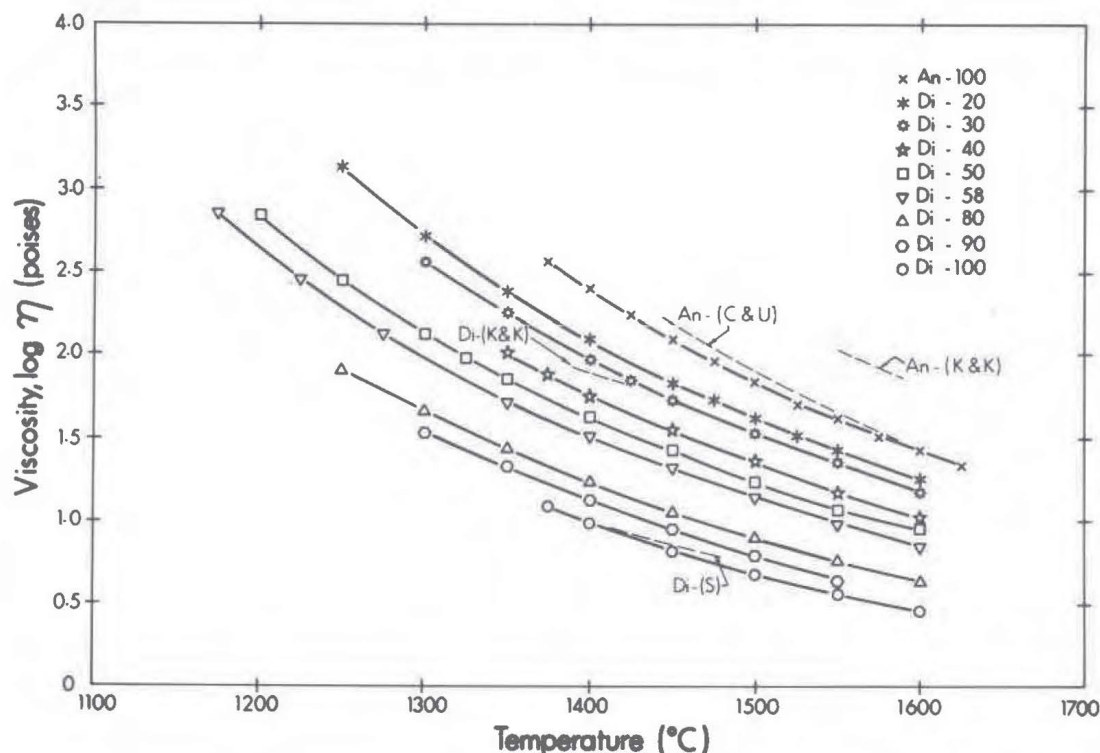
Fig. 1. Viscosity-temperature plot for compositions in the system diopside-anorthite. Dashed lines are previous determinations by Kozi and Kani (1935), Cukierman and Uhlmann (1973), and Scarfe et al. (1979). Liquidus temperatures for each composition are given in Table 2.
