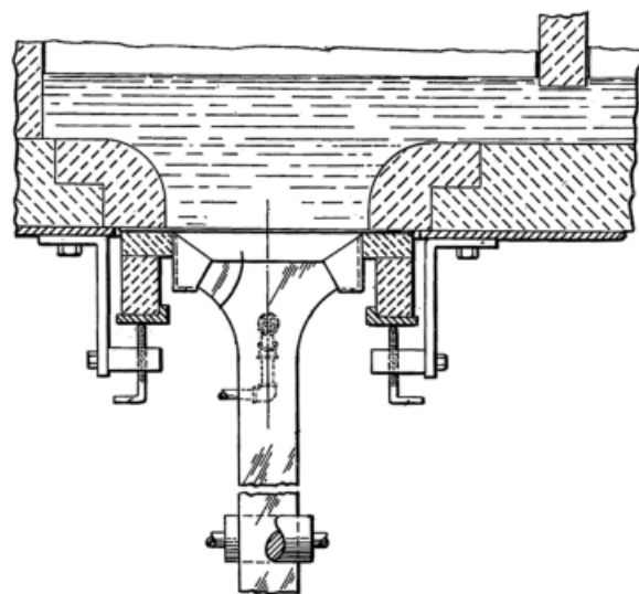
Fig. 1. The slot draw-forming apparatus as envisioned by Brown. 17 The molten glass collects in a receptacle above the slot. The shape of the slot keeps the glass from becoming too thin at the edges by supplying additional glass at an angle with respect to the pull direction. The continuous glass ribbon is pulled by pulling rolls, and can be cut to size or passed through an annealer below the rolls.
