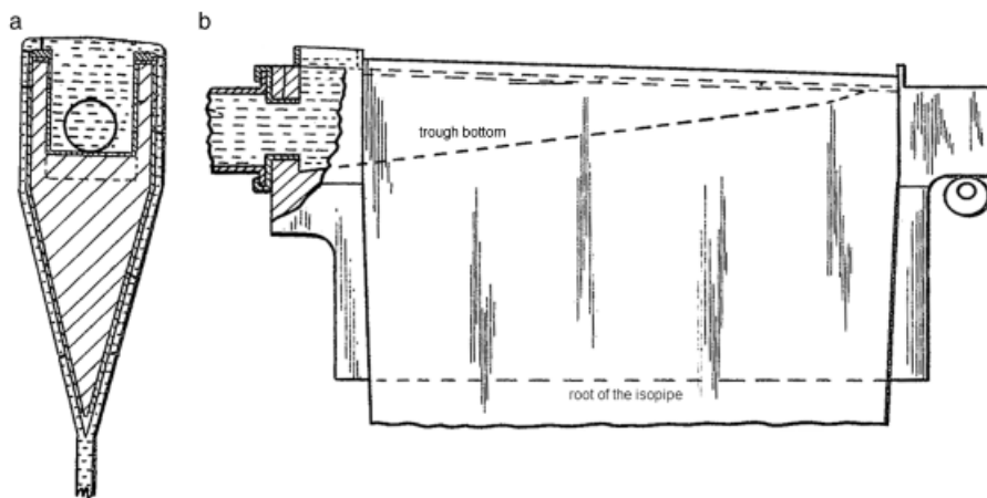
Fig. 2. (a) A cut-away drawing of an isopipe, the forming anvil used in the fusion draw process. 20 The diagonal lines indicate the refractory, and the horizontal dotted lines represent glass. The refractory trough at the top of the figure is defined by the weir walls. Glass overflows the weirs, flows down either side of the refractory, and joins at the base, or root. (b) The isopipe is seen perpendicular to the face of a sheet. The dashed line near the bottom represents the root, or base of the refractory. The trough (diagonal dash line increasing from left to right) is deeper at the left (inlet) than at the right to ensure uniform glass flow over the walls of the trough.
