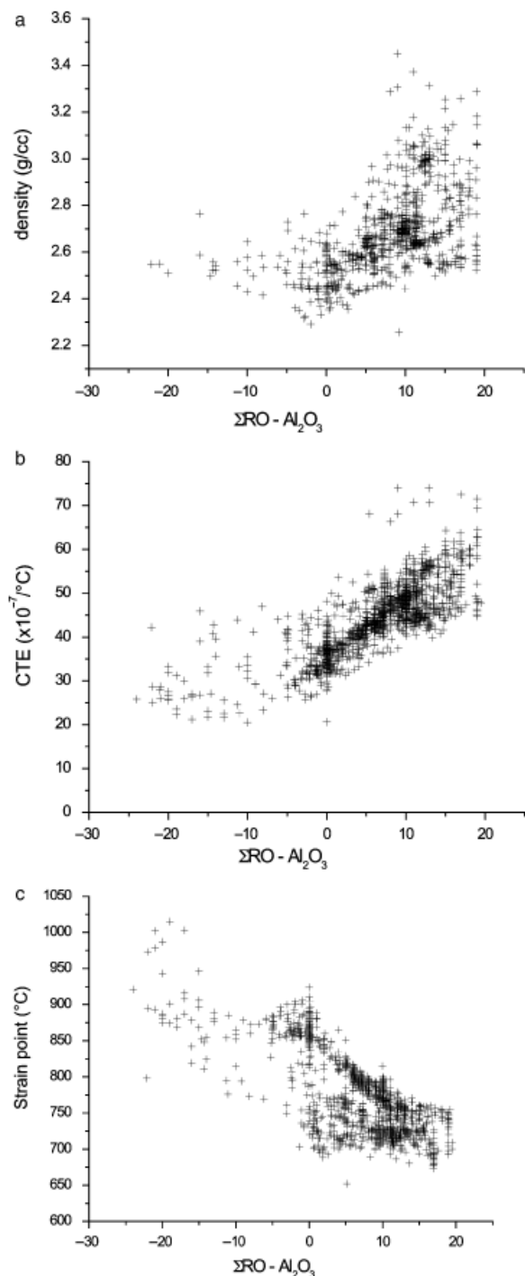
Fig. 3. (a) Density ( \text{g/cm}^3 ) versus \Sigma\text{RO}-\text{Al}_2\text{O}_3 for alkaline earth borosilicate glasses, in which \Sigma\text{RO} represents the sum of the mole percents of the alkaline earth oxides ( \text{MgO} , \text{CaO} , \text{SrO} , and \text{BaO} ). \Sigma\text{RO} ranges from 0 to 20 mol%, \text{B}_2\text{O}_3 from 0 to 18 mol%, \text{SiO}_2 from 50 to 80 mol%, and \text{Al}_2\text{O}_3 from 4 to 34 mol%. (b) Coefficient of thermal expansion ( \text{RT}-300^\circ\text{C} ) versus \Sigma\text{RO}-\text{Al}_2\text{O}_3 for the alkaline earth borosilicate glasses referenced in (a) (c) Strain point versus \Sigma\text{RO}-\text{Al}_2\text{O}_3 for the alkaline earth borosilicate glasses referenced in (a).
