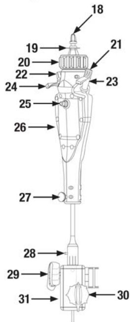
Figure 4: CDS Handles
