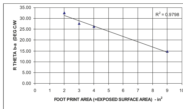
Figure 4. R\Theta_{B-A} Board-Ambient per Emitter vs. Foot Print Area
