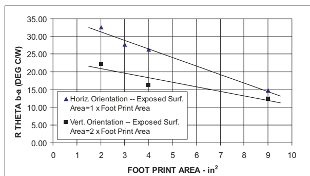
Figure 5. R_{\theta_{B-A}} per Emitter in Free Convection Vs. Foot Print Area.
