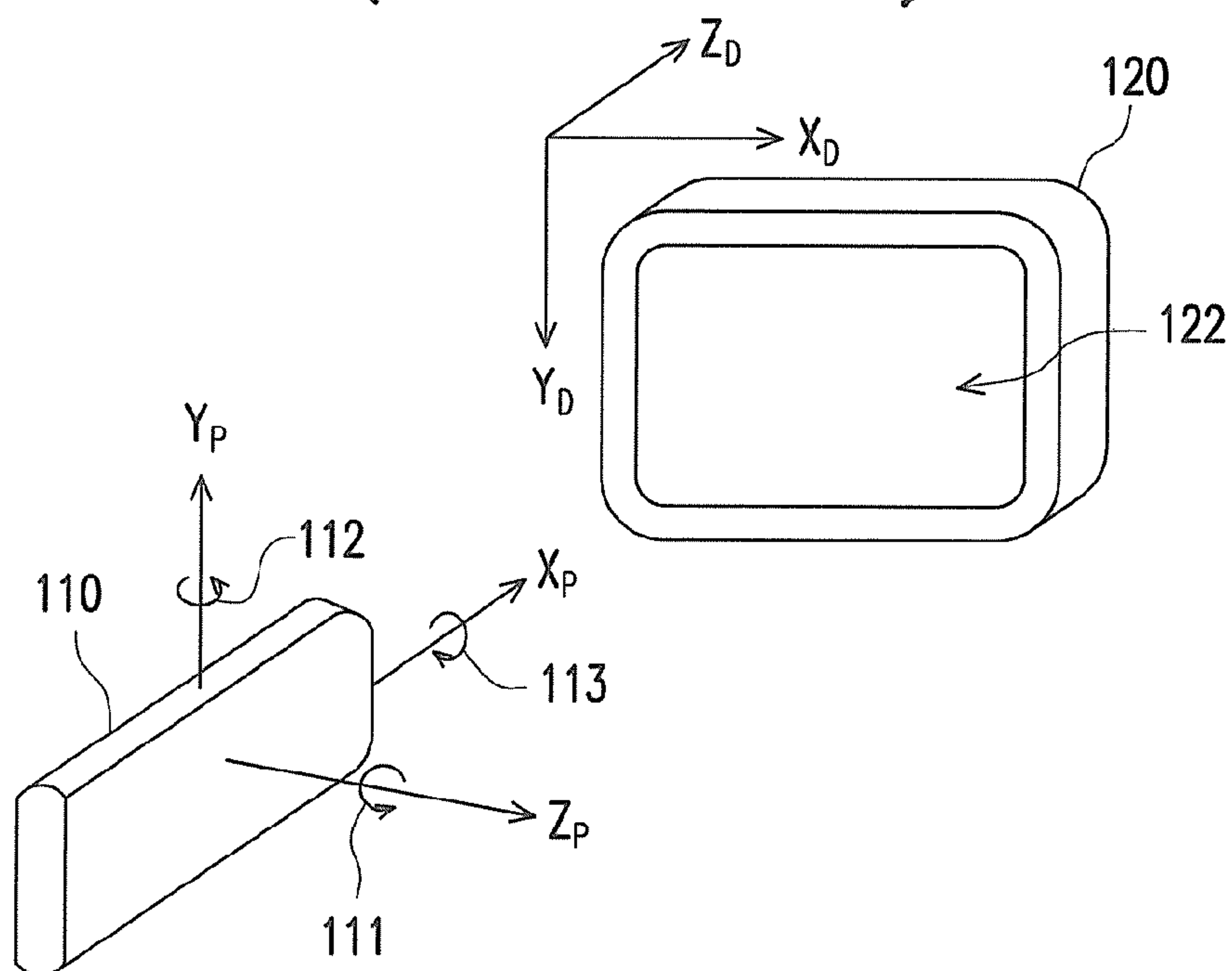
FIG. 1 (RELATED ART)
