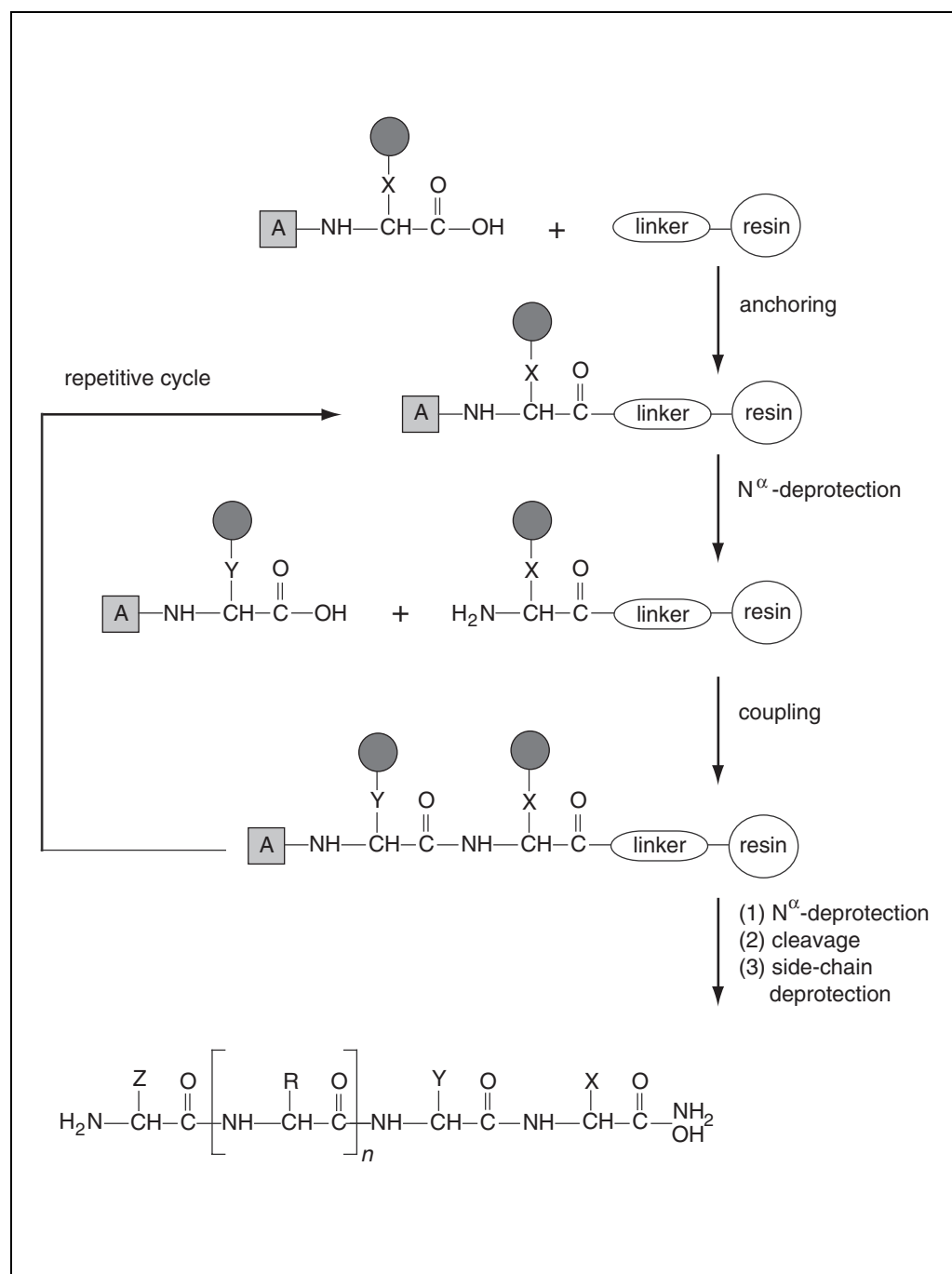
Figure 18.1.1 Generalized approach to solid-phase peptide synthesis. Symbols: A, N^\alpha -protecting group; circle, side-chain protecting groups; R, X, Y, and Z, side-chain functionalities.
