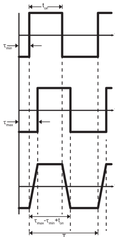
Figure 8.3.3: The effect of dispersion on the signal output from the fiber optic cable: Top: Arriving waveform corresponding to minimum path length, Middle: Arriving waveform corresponding to maximum path length, and Bottom: Sum of all arriving waveforms. (CC BY-SA 4.0; S. Lally)
