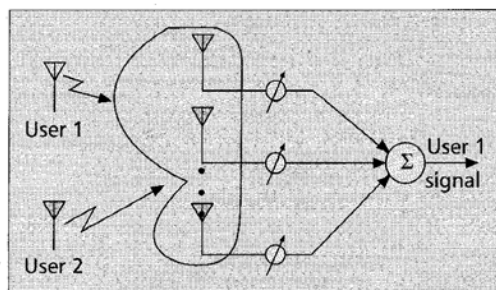
■ Figure 4. An adaptive array beam pattern in a line-of-sight system.
