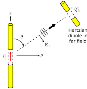
Figure 10.11.2: The dipole of interest driven by current \tilde{I}_1^t radiates electric field \tilde{\mathbf{E}}_1 , resulting in open-circuit potential \tilde{V}_2^r at the terminals of a Hertzian dipole in the far field. (CC BY-SA 4.0; C. Wang)
