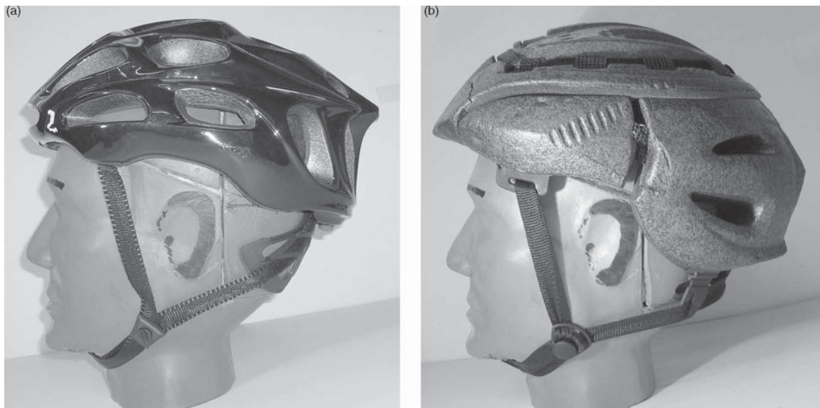
Fig. 7 Coverage of an Ogle headform: (a) S1 and (b) Sportcraft helmets
