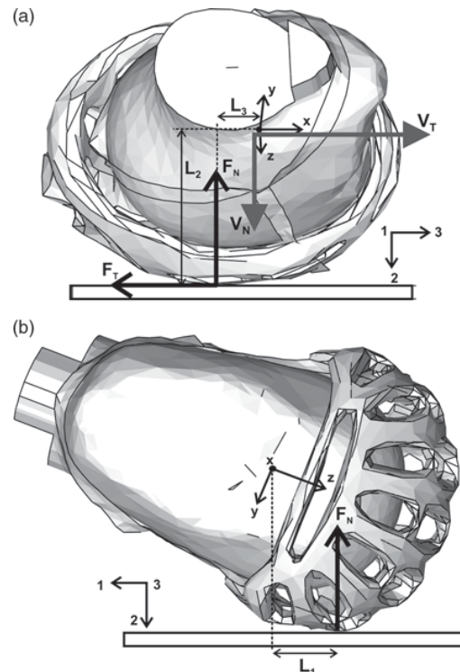
Fig. 1 Oblique impact on the left 70° site of a S1 helmet, showing the axes xyz through the headform centre of gravity and road axes 123. L_i are the offsets of the lines of action of the normal F_N and tangential F_T forces from the headform centre of gravity
