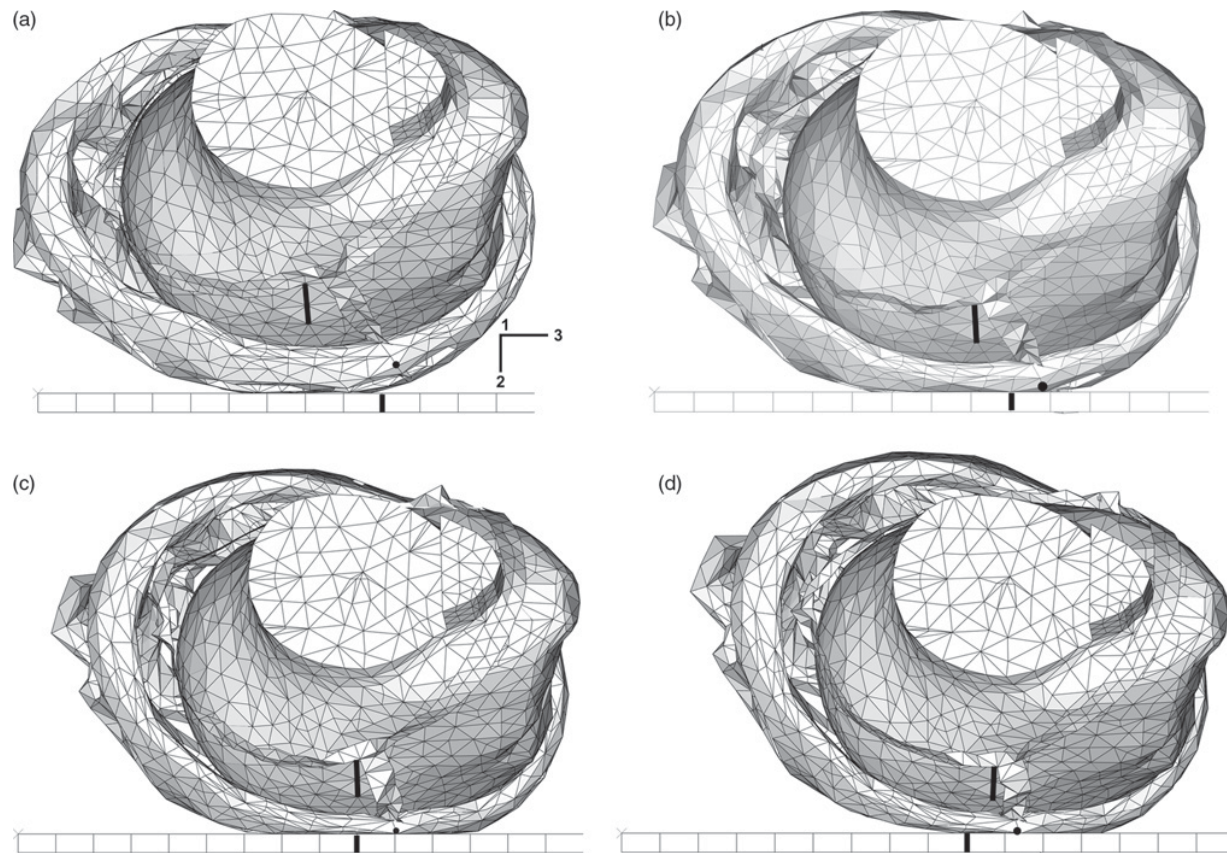
Fig. 4 2, 3 plane view of a S1 helmet oblique impacted on the left 70^\circ site, with velocity components V_N = 5.4 and V_T = 10.0 m/s, at times: (a) 1.8 ms, (b) 4.0 ms, (c) 6.0; and (d) 7.8 ms since initial road contact
