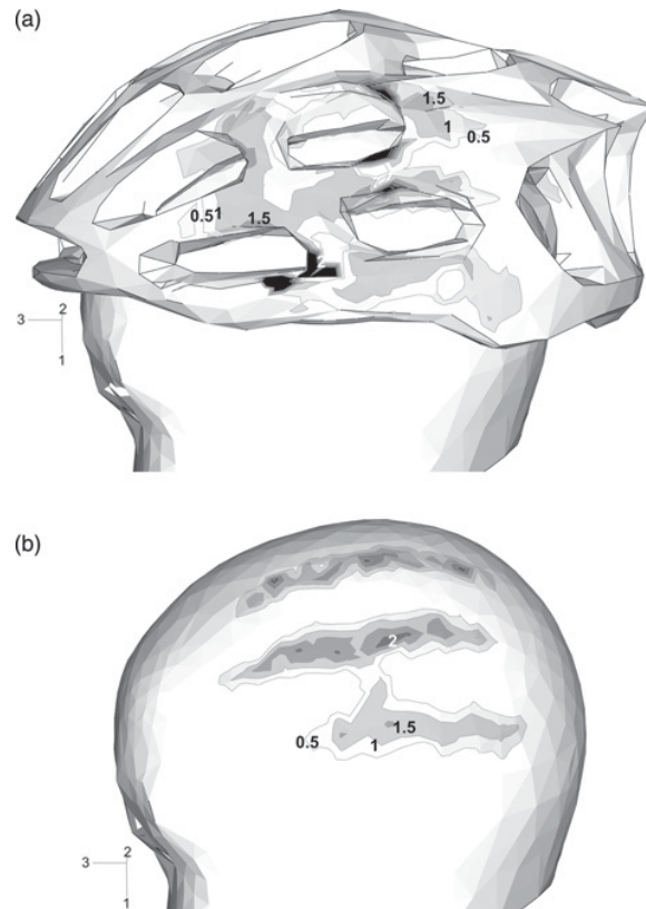
Fig. 10 Contours of pressure \sigma_{22} (MPa) after 5.0 ms of an oblique impact with V_N = 5.4 and V_T = 4.0 m/s at the left 70^\circ site of a S1 helmet: (a) on the liner exterior and (b) on the deformable headform
