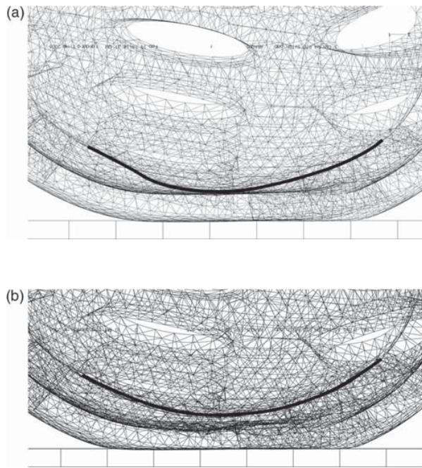
Fig. 3 Wireframe views in the 2, 3 plane of two-layer helmet liners after 3.6 ms, for impacts with V_N = 5 and V_T = 10.0 m/s on the left 70^\circ site: (a) inner 35 \text{ kg/m}^3 density liner and outer 83 \text{ kg/m}^3 liner, and (b) two liners of 55 \text{ kg/m}^3 density (inner surface of inner liner is emphasised)
