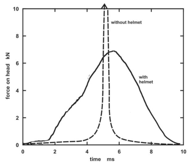
Fig. 6 Head impact force versus time trace with (based on FEA) and without (schematic) a helmet. The areas under the curves (the impulses) are the same
