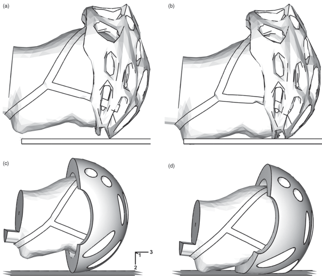
Fig. 8 FEA predictions for oblique impacts with V_N = 5.4 and V_T = 5 m/s at the frontal 90^\circ site: (a) S1 helmet at initial contact, (b) after 3.2 ms, with forehead-to-road impact, (c) 16-hole helmet initially, and (d) after 8.4 ms
