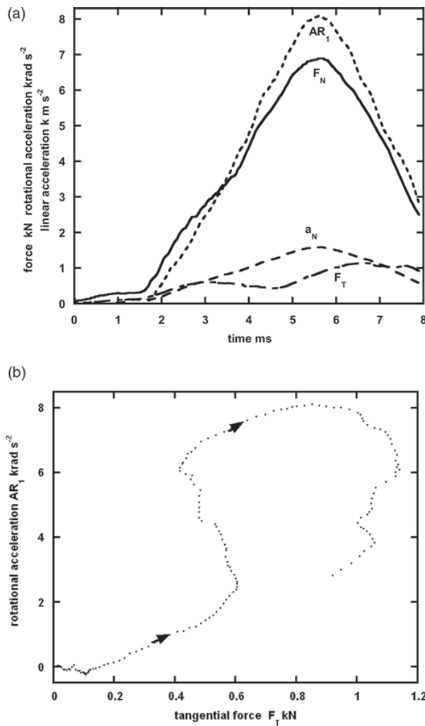
Fig. 5 For the simulation of Fig. 2: (a) road forces and headform accelerations versus time and (b) correlation of head rotational acceleration about the 1 axis, with the tangential force F_T
