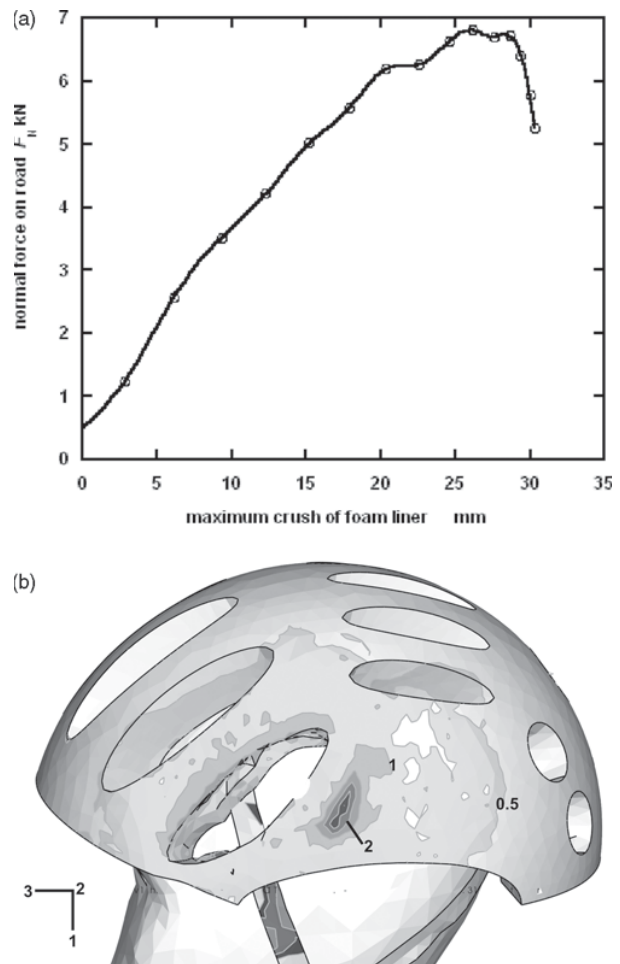
Fig. 2 Impact of 16-hole helmet with V_N = 5 and V_T = 10.0 \text{ m/s} on the left 70^\circ site: (a) variation of the normal force F_N with the foam crush distance in the centre of the impact region, and (b) contours of pressure \sigma_{22} (MPa) on the liner at the peak of the impact
