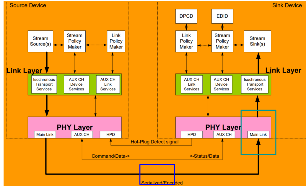
Figure 1-2: Layered Architecture
