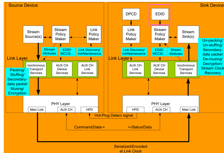
Figure 2-1: Overview of Link Layer Services
