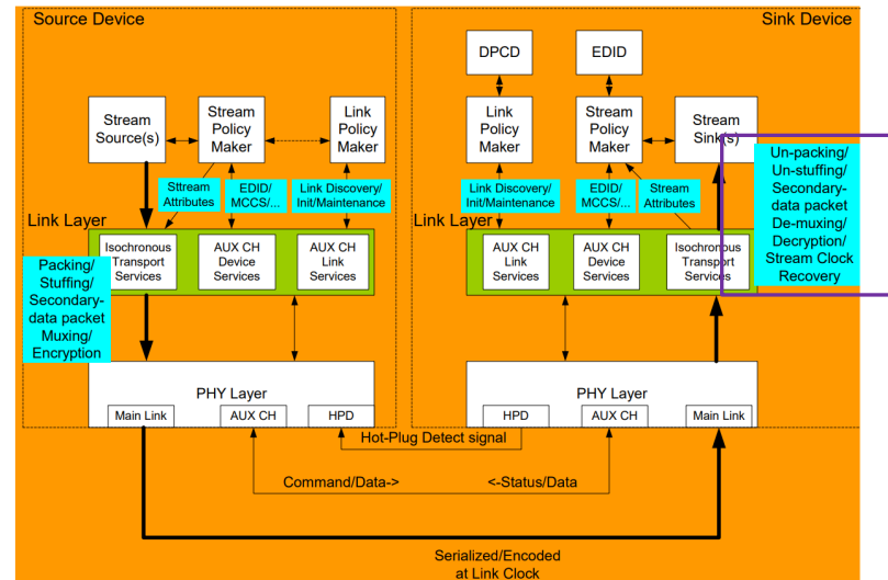
Figure 2-1: Overview of Link Layer Services
