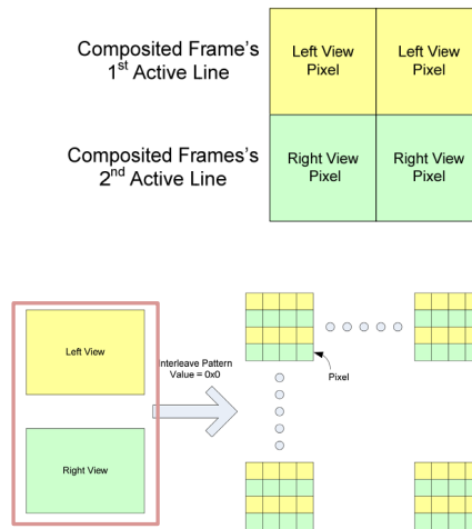
Figure 2-29: Interleave Pattern Corresponding to 2-way Interleaved Stereo where Right Image Pixels are on Even Lines
