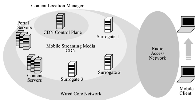
Fig. 2 Basic architecture of mobile streaming media CDN.
