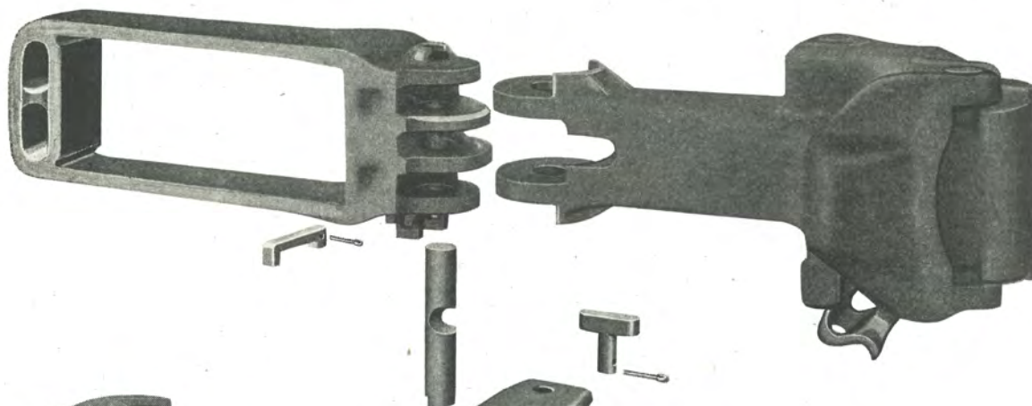
Fig. 10.100—Buckeye A.A.R. vertical-plane draft yoke of high-tensile steel.
