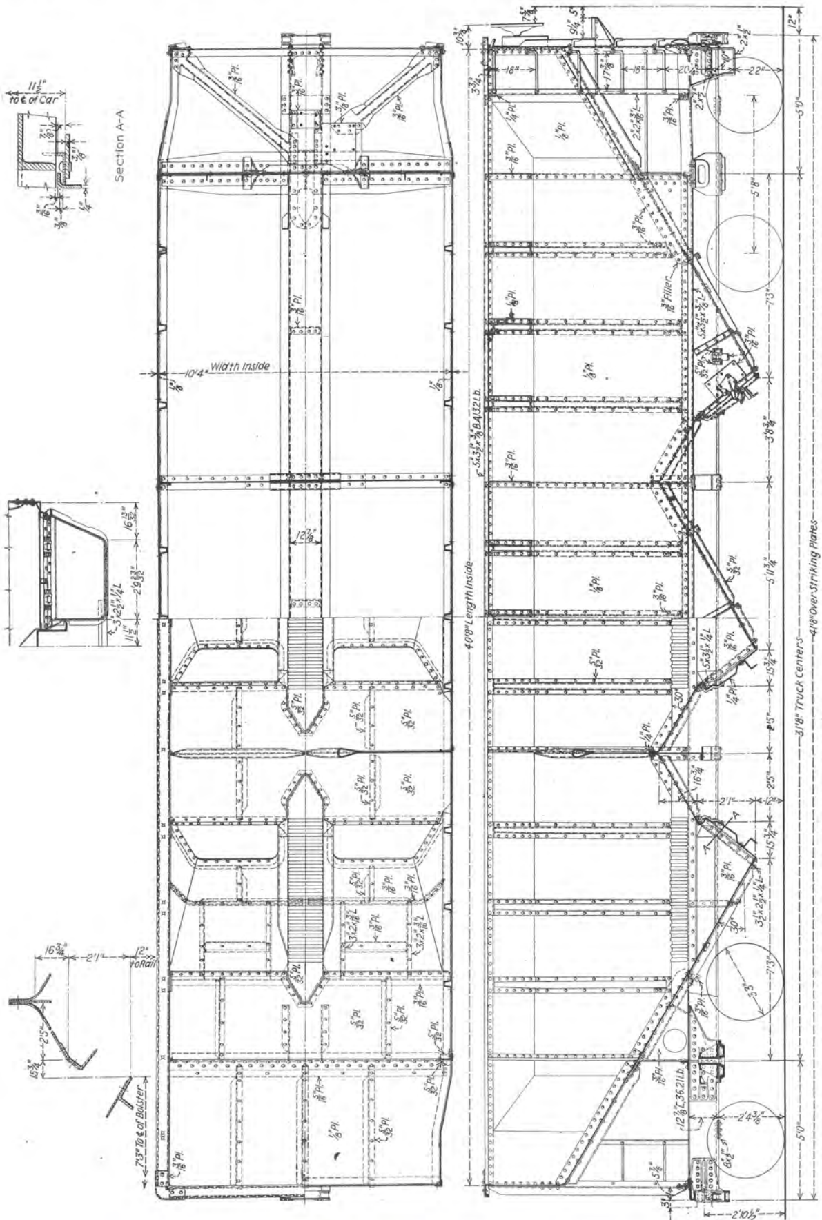
Fig. 2.637—Bessemer & Lake Erie 90-ton triple hopper car, light weight (USS Cor-Ten steel). 6½ in. x 12 in. Journal Axles, Road Class HT17. (Note—Cars of 70 tons capacity were also built. These differed only in having trucks with 6 in. x 11 in. axles—See Fig. 2.640) (See also Page 277)
