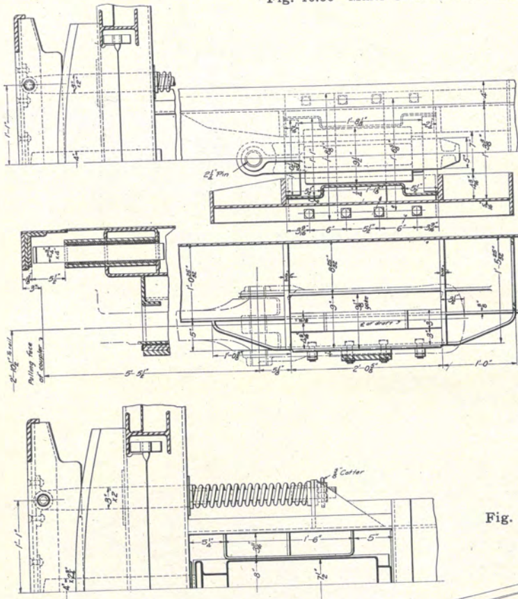
Fig. 10.60—Miner Class A-28-XB draft gear applied to caboose car.
