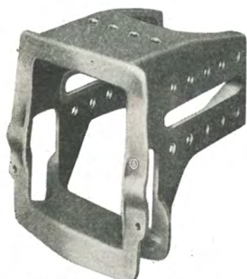
Fig. 10.102—Striker with Integral Front Lugs and Swing Coupler Carrier.
