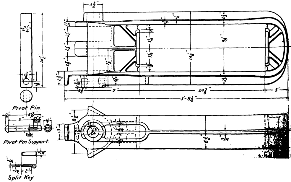
Fig. 10.127—Cast steel yoke for passenger service in combination with Type E Couplers. Pivot pin in quadruple shear.
