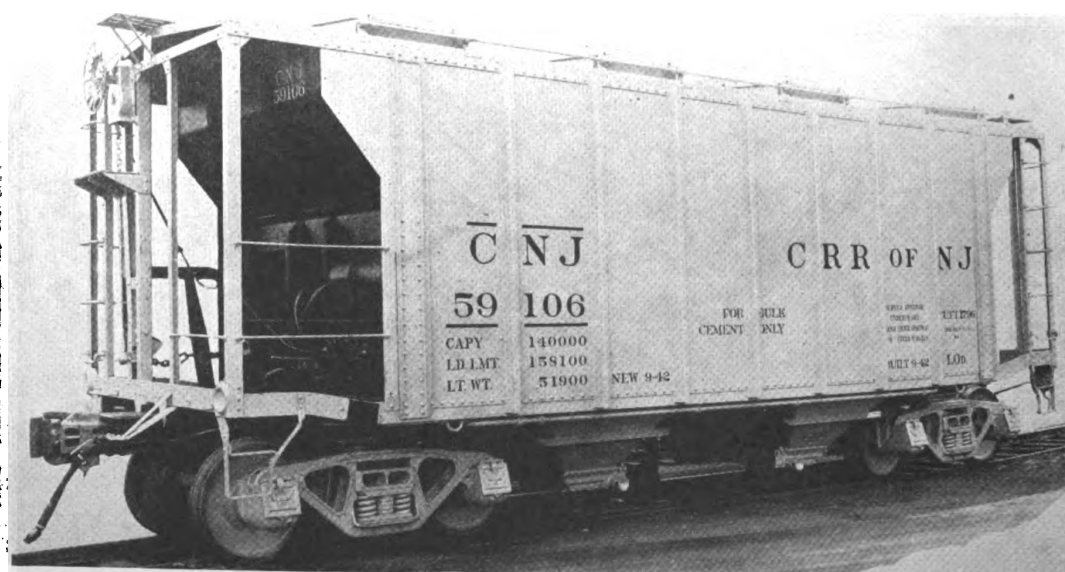
Fig. 2.691 —C. R. R. of N. J. 70-ton covered hopper car with Duryea cushion underframe. Builder, American Car and Foundry Co. Capacity, 1,796 cu. ft.; light weight, 51,900 lb.; load limit, 158,100 lb.; inside, length 26 ft. 3 in.; width 9 ft. 8 in.; height over running board 12 ft. 11 in.
