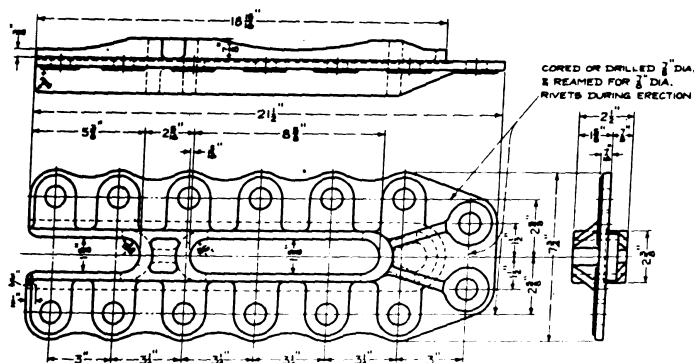
Fig. 10.113—Cheek plate for Farlow draft gear attachments.
