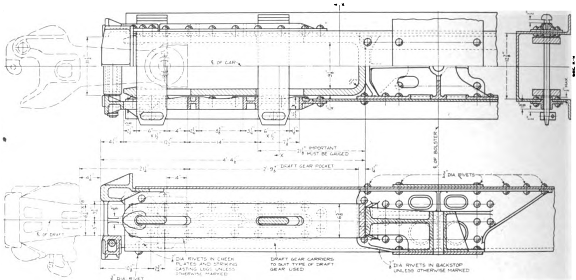
Fig. 10.119—Application of Symington selective travel draft gear attachments.
