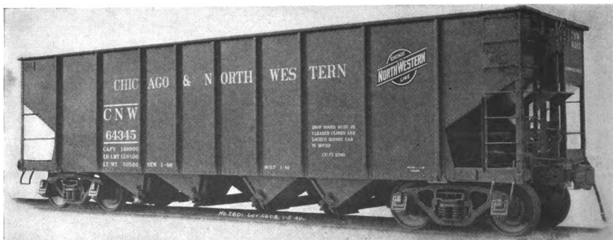
Fig. 2.651 —Chicago & North Western 70-ton capacity quadruple hopper car, A. A. R. Class HT. Builder, Pullman-Standard Car Manufacturing Company.
