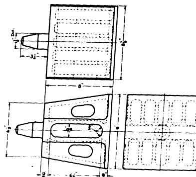
Fig. 10.114—Follower block.
