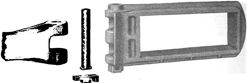
Fig. 10.125—Cast steel yoke with quadruple shear pivot pin.
