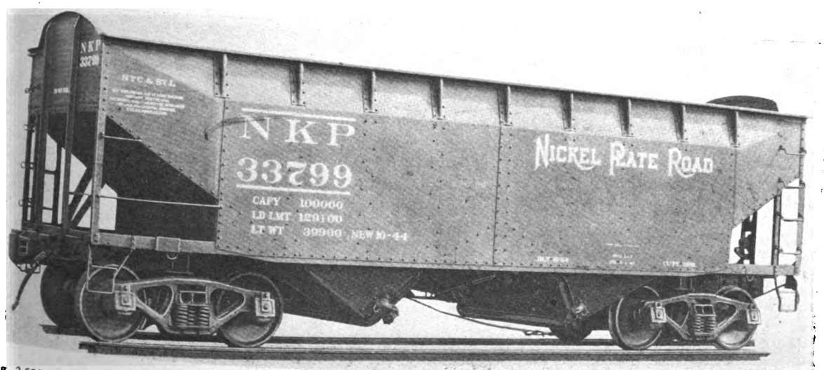
Fig. 2,621—New York, Chicago & St. Louis (Nickel Plate) 50-ton twin hopper coal car. Builder, American Car and Foundry Co. Light weight, 39,900 lb.; load limit, 129,100 lb.; capacity, 2,081 cu. ft.; inside, length 33 ft. 0 in.; width 10 ft. 4 in.; height of sides 10 ft. 6 in.
