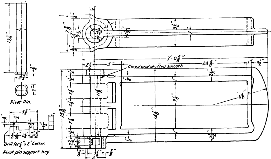
Fig. 10.126—Cast steel yoke for passenger service. Pivot pin in quadruple shear.
