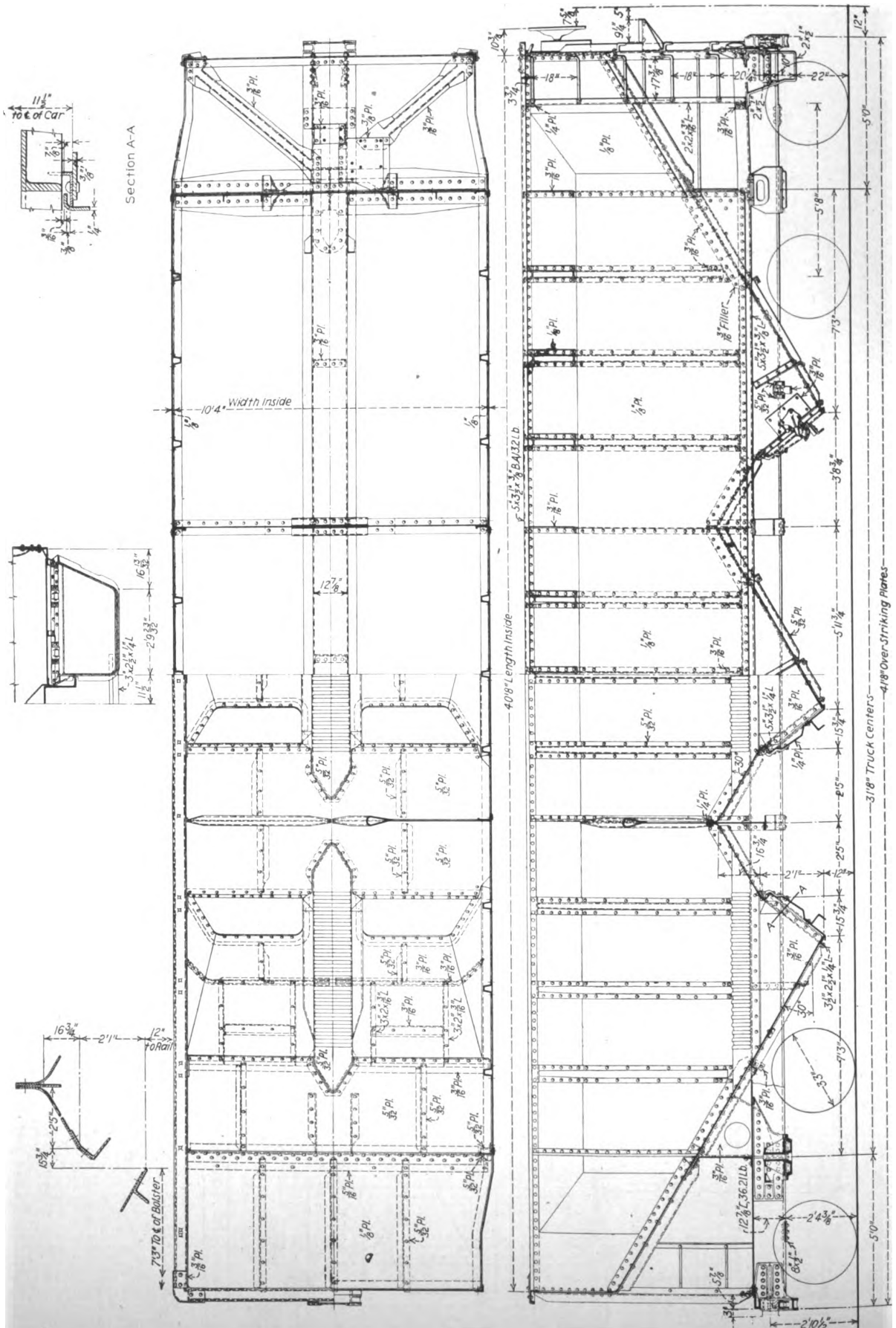
Fig. 2.637—Bessemer & Lake Erie 90-ton triple hopper car, light weight (USS Cor-Ten steel). 6 1/2 in. x 12 in. Journal Axles. Road Class HT17. (Note—Cars of 70 tons capacity were also built. These differed only in having trucks with 6 in. x 11 in. axles—See Fig. 2.640) (See also Page 277)
