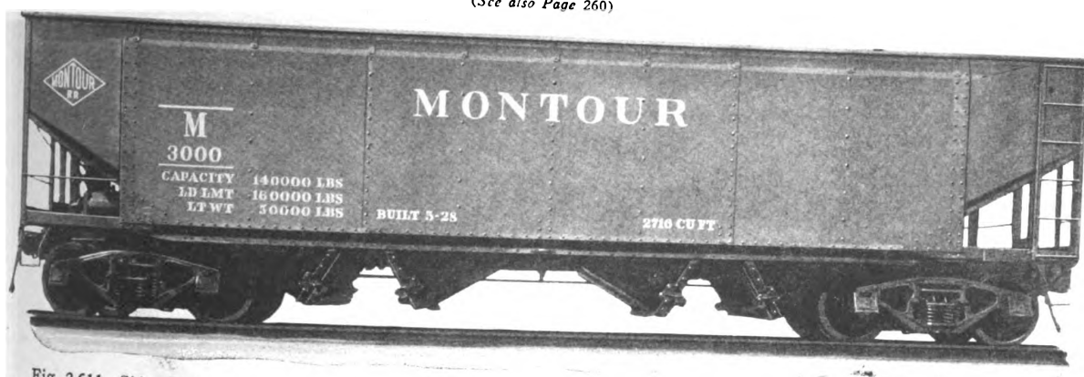
Fig. 2.611—Side view of 70-ton hopper car using Unitcast design cast steel body bolsters, crossbearers and hopper frames.
