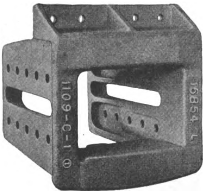
Fig. 10.109 —Combined striking casting and front draft lugs.
