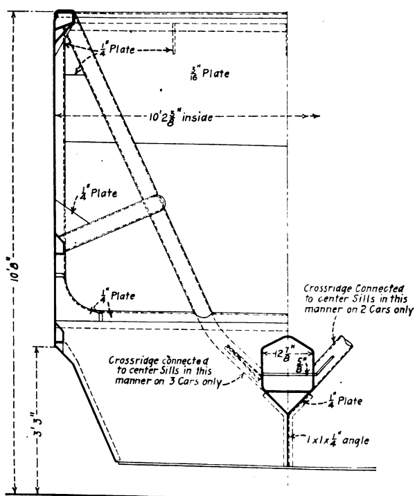
Fig. 2.642 —Cross section of C. G. W. all-welded hopper car.
