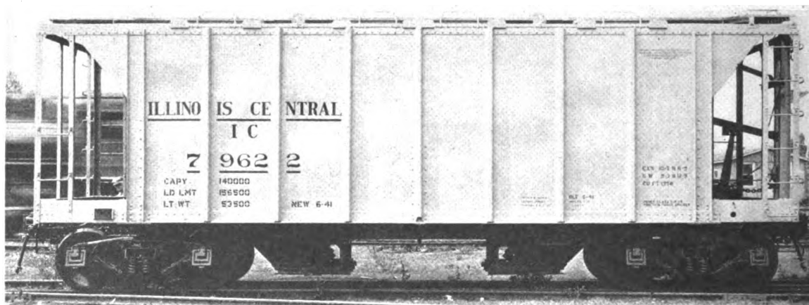
Fig. 2.689 —Illinois Central 70-ton covered hopper car. Builder, General American Transportation Corp. Capacity, 1,958 cu. ft.; light weight, 53,500 lb.; load limit, 156,500 lb.; inside, length 29 ft. 3 in.; width 9 ft. 5½ in.; height over running board 12 ft. 9¾ in.
