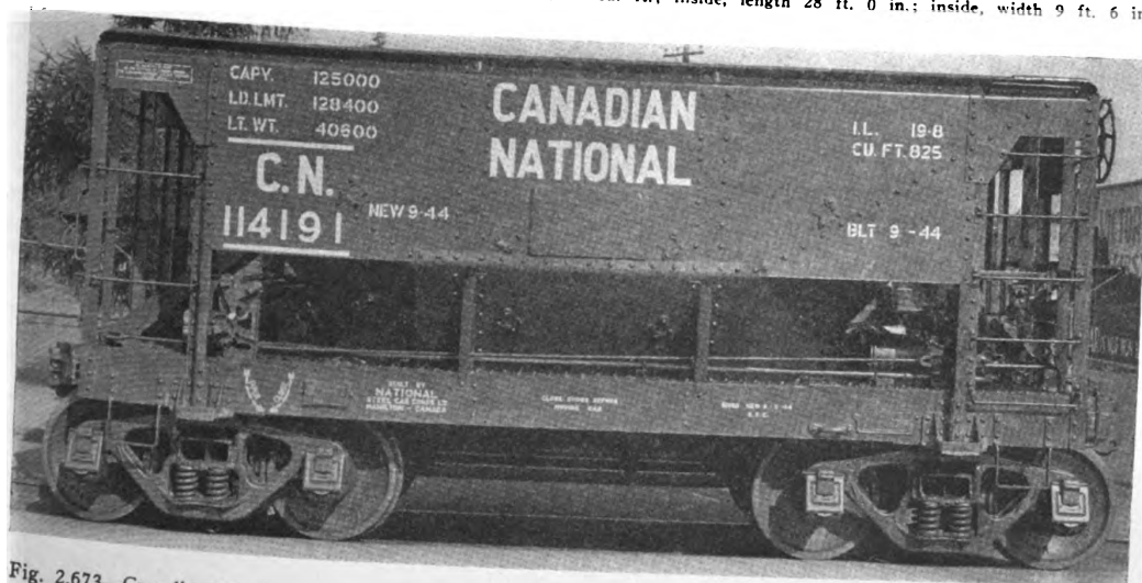
Fig. 2.673—Canadian National 50-ton center discharge ore car for use at Steep Rock mining operations. Built by National Steel Car Corporation, Ltd. Light weight, 40,600 lb.; load limit, 128,400 lb.; capacity, 825 cu. ft.; length inside, 19 ft. 8 in. (See also page 294)
