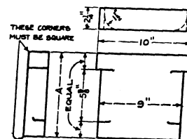
Fig. 10.114—Follower block.
