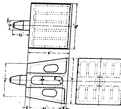
Fig. 10.114—Follower block.
