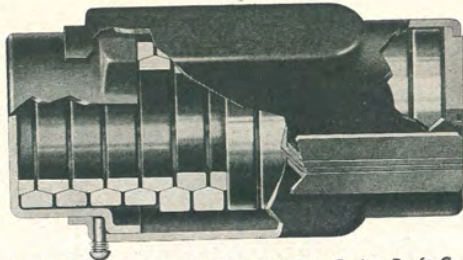
Fig. A—Sectional view of Edgewater Ring Spring Draft Gear
