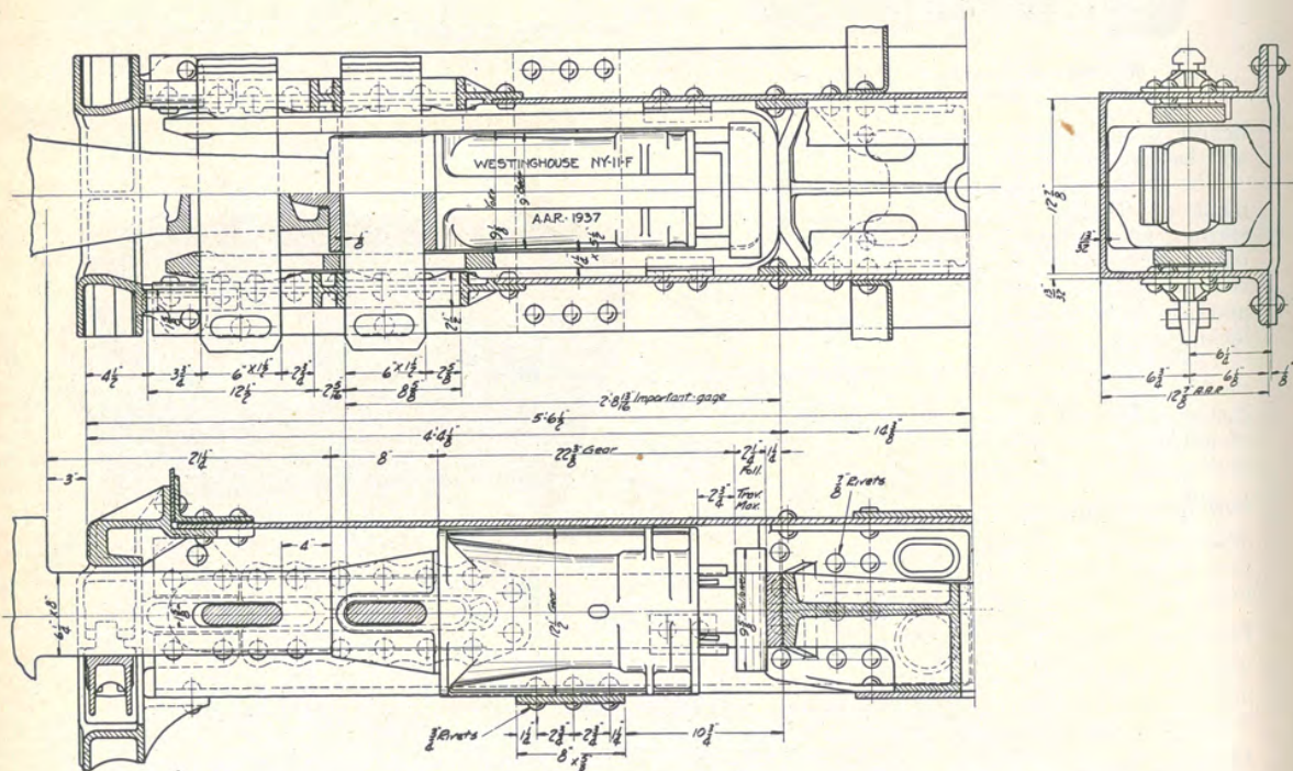
Fig. 10.52—Application of Westinghouse Type NY-11-F friction draft gear with horizontal yoke.
