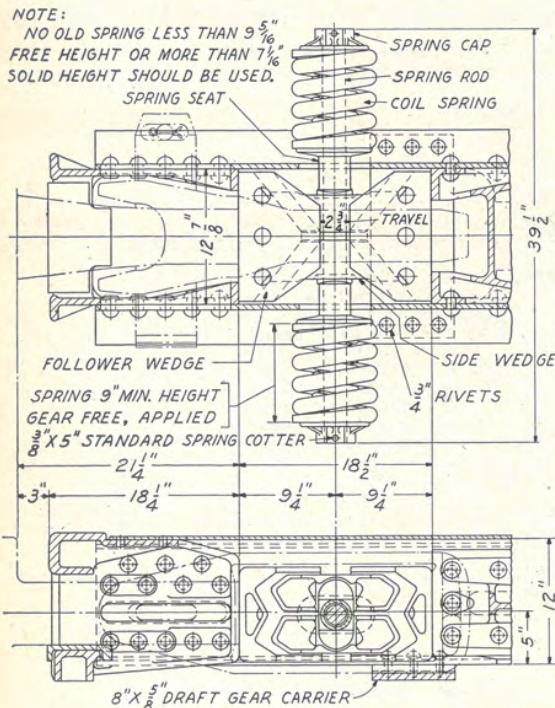
Fig. 10.82—Peerless Type "KC" friction draft gear.
