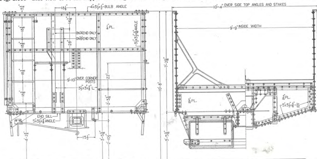
Fig. 2.612—End elevation and half cross-sections of Unitcast design 55-ton twin hopper car incorporating cast steel crossbearer arms, body bolster center, center sill hood ends and hopper frames. (See also Page 262)
