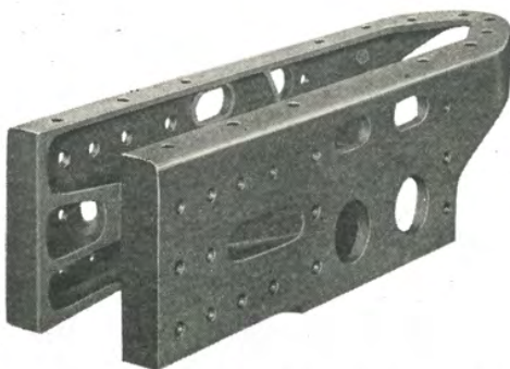
Fig. 10.104—Bolster Center Filler and Rear Draft Gear Lugs for box car.
