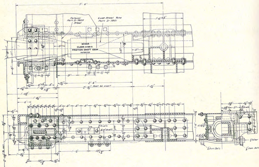
Fig. 10.59 —Miner Class A-98-X friction draft gear applied to freight equipment.
