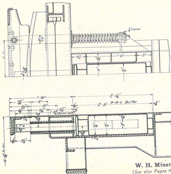
Fig. 10.62—Miner Class B-18-X friction buffer applied to passenger equipment.
