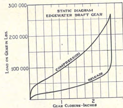
Fig. B—Typical force-closure diagram of Edgewater Ring Spring Draft Gear
