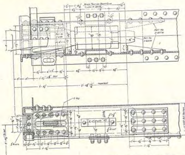
Fig. 10.60—Miner Class A-28-XB draft gear applied to caboose car.
