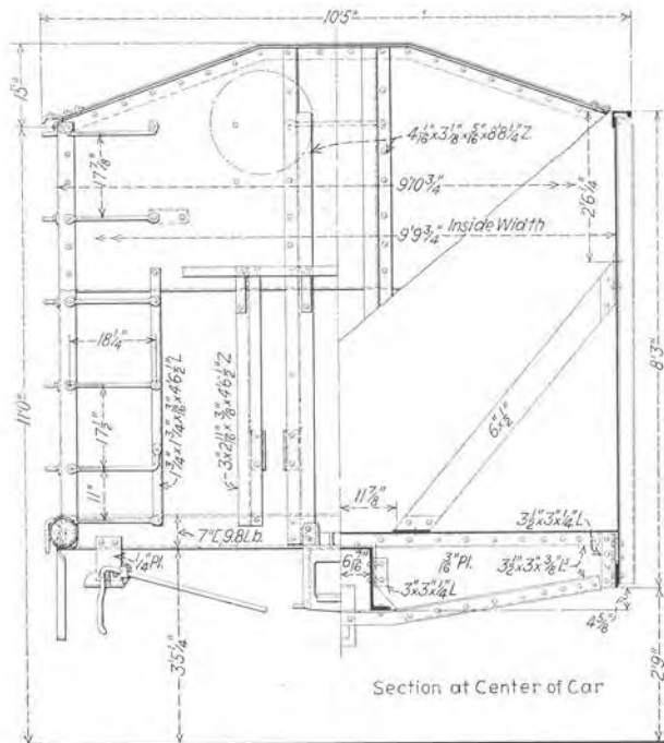
Fig. 2.606—End view and cross section of Norfolk & Western Class HL hopper car shown on Page 258.
