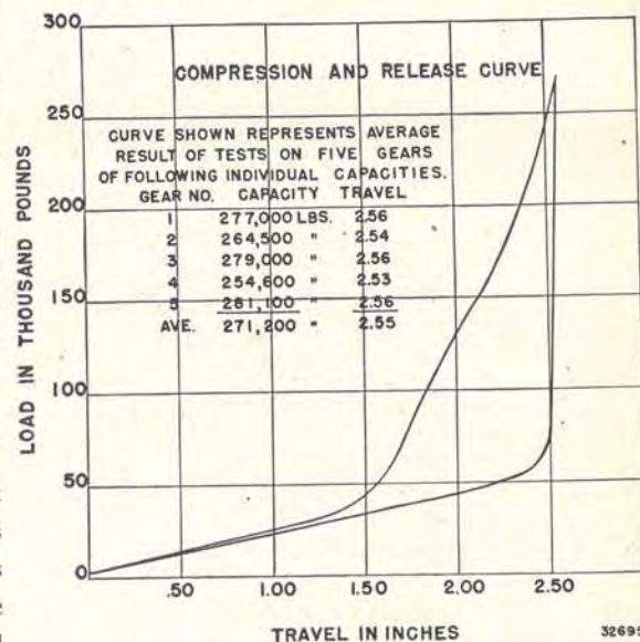
Fig. D—Closure Chart for Type K-4 Gears
